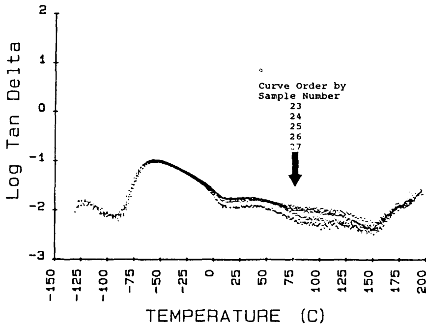
Figure 11. \text{Tan } \delta for unstretched material, Samples 23 through 27.
