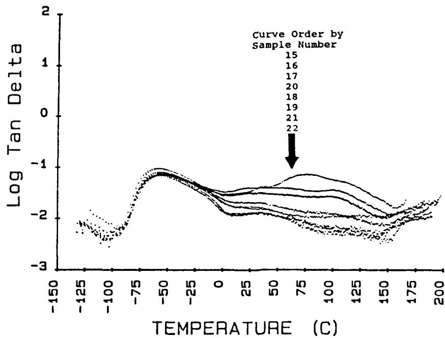
Figure 9. Tan \delta for unstretched material, Samples 15 through 22.
