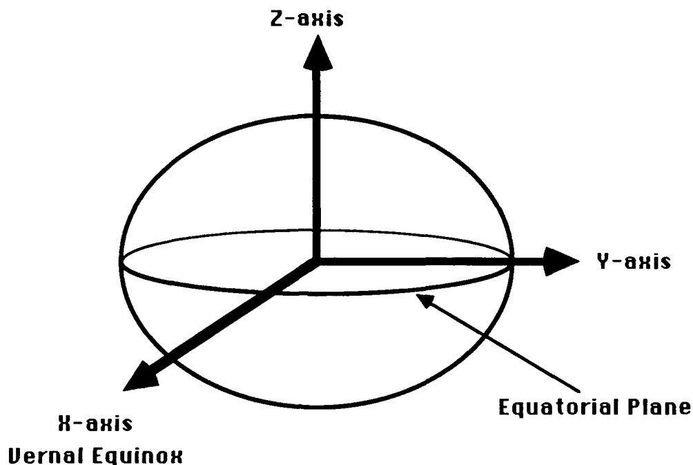
Figure A.1. Earth Centered Inertial Coordinate System
