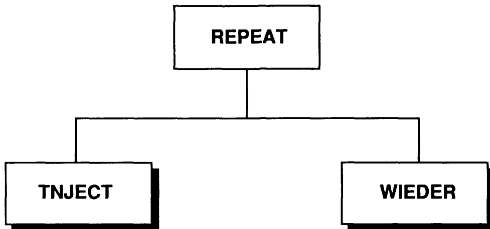
Figure 3.2. Subroutine REPEAT
