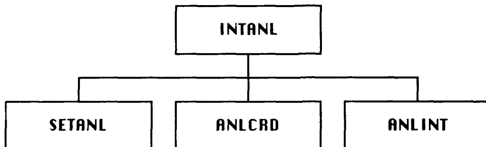
Figure 2.2. Subroutine INTANL
