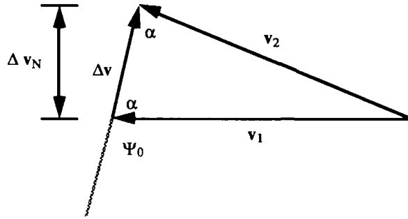
Figure 4.7. Velocity Vectors in Normal and Tangential Planes
