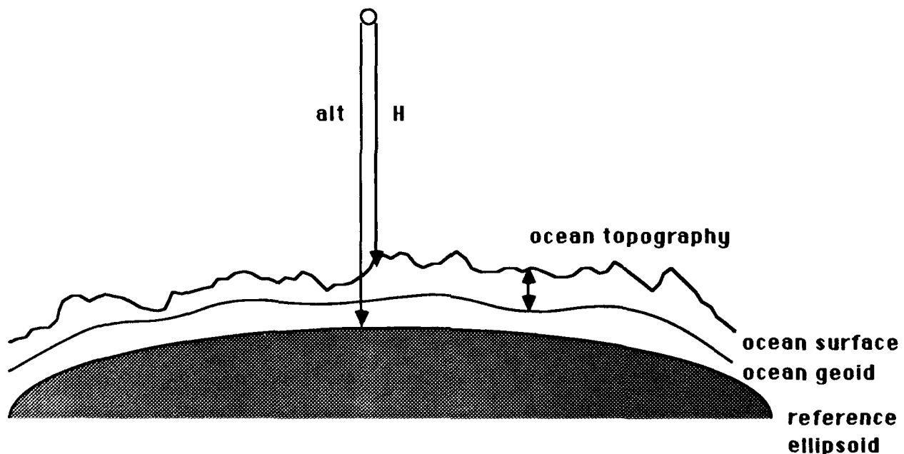
Figure 1.1. Illustration of Sea Surface Topography
