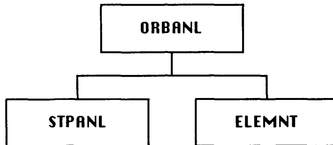
Figure 2.3. Subroutine ORBANL
