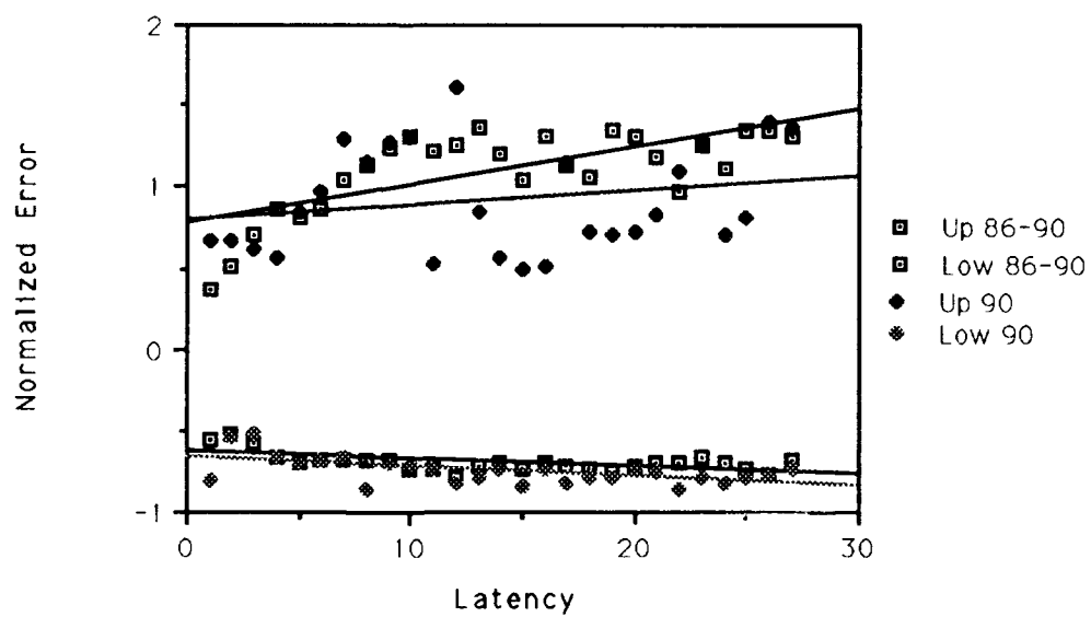
Figure 5.3. Upper and Lower Limits of Confidence Interval
