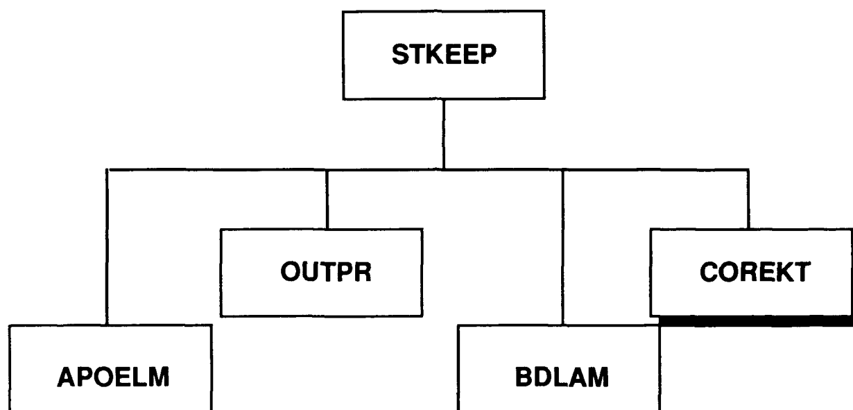
Figure 3.3. Subroutine STKEEP
