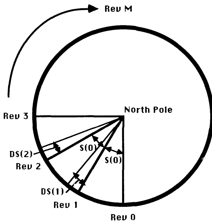
Figure 4.2. Node Drift
