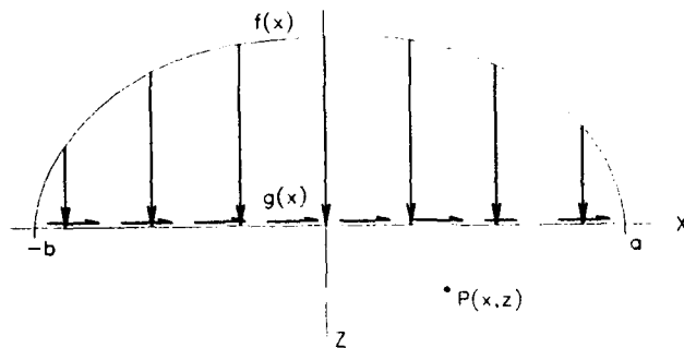
Figure 2. Elastic Half-Space with a Normal and Tangential Loading Distribution
