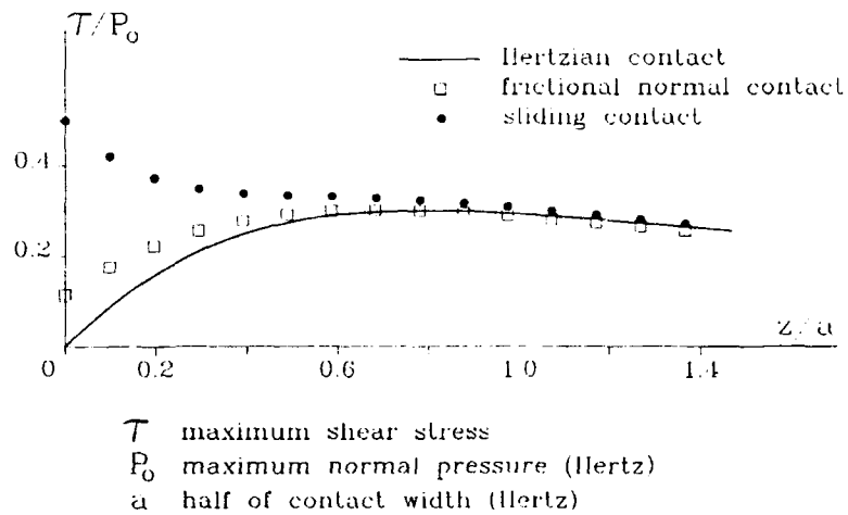
Figure 11. Shear Stress Distributions on the Aluminum Cylinder
