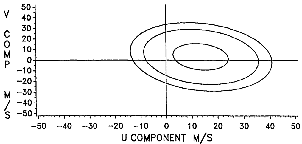
Figure E-40. Wind Probability Ellipses, January, 12 KM.
