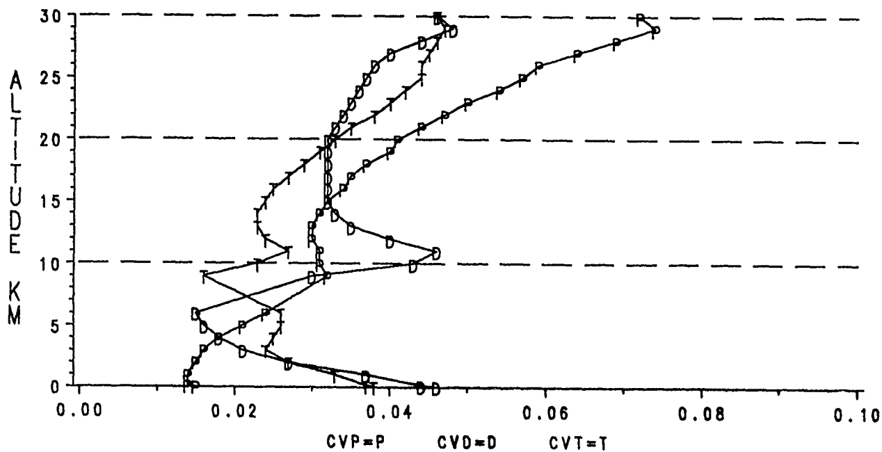
Figure F-17. Coefficients of Variation for Pressure (P), Density (D), and Temperature (T), January.
