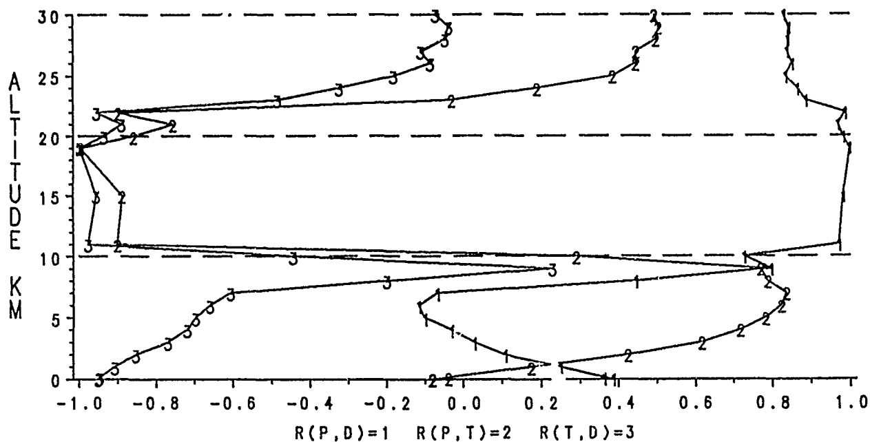
Figure F-20. Correlation Coefficients for P&D, P&T, and T&D, July.
