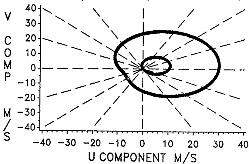
Figure E-21. Wind Interpercentile Range and Mean, January, 8 KM.
