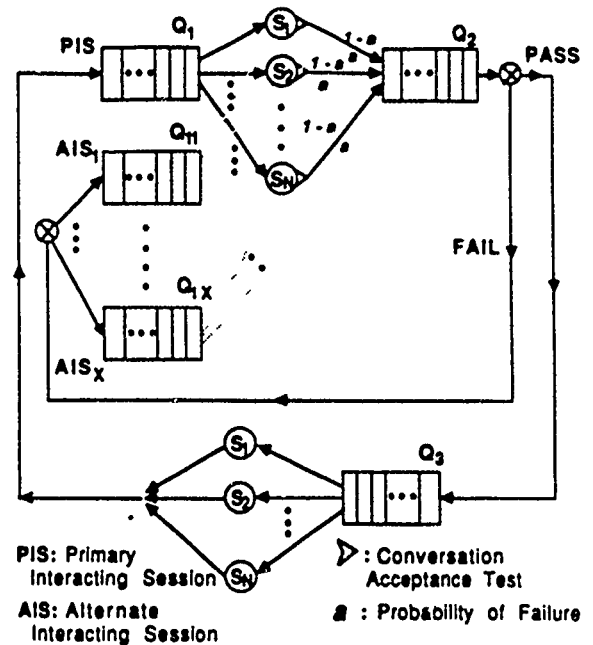
Fig. 4. A queueing network model of the system in Fig. 2.
