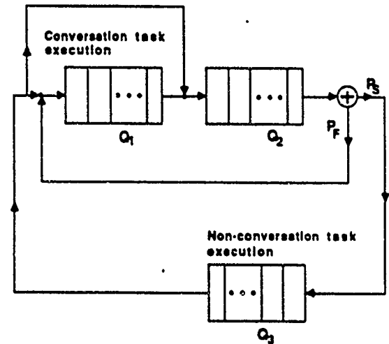
Fig. 5. An abstract representation of the queueing network model in Fig. 4.
