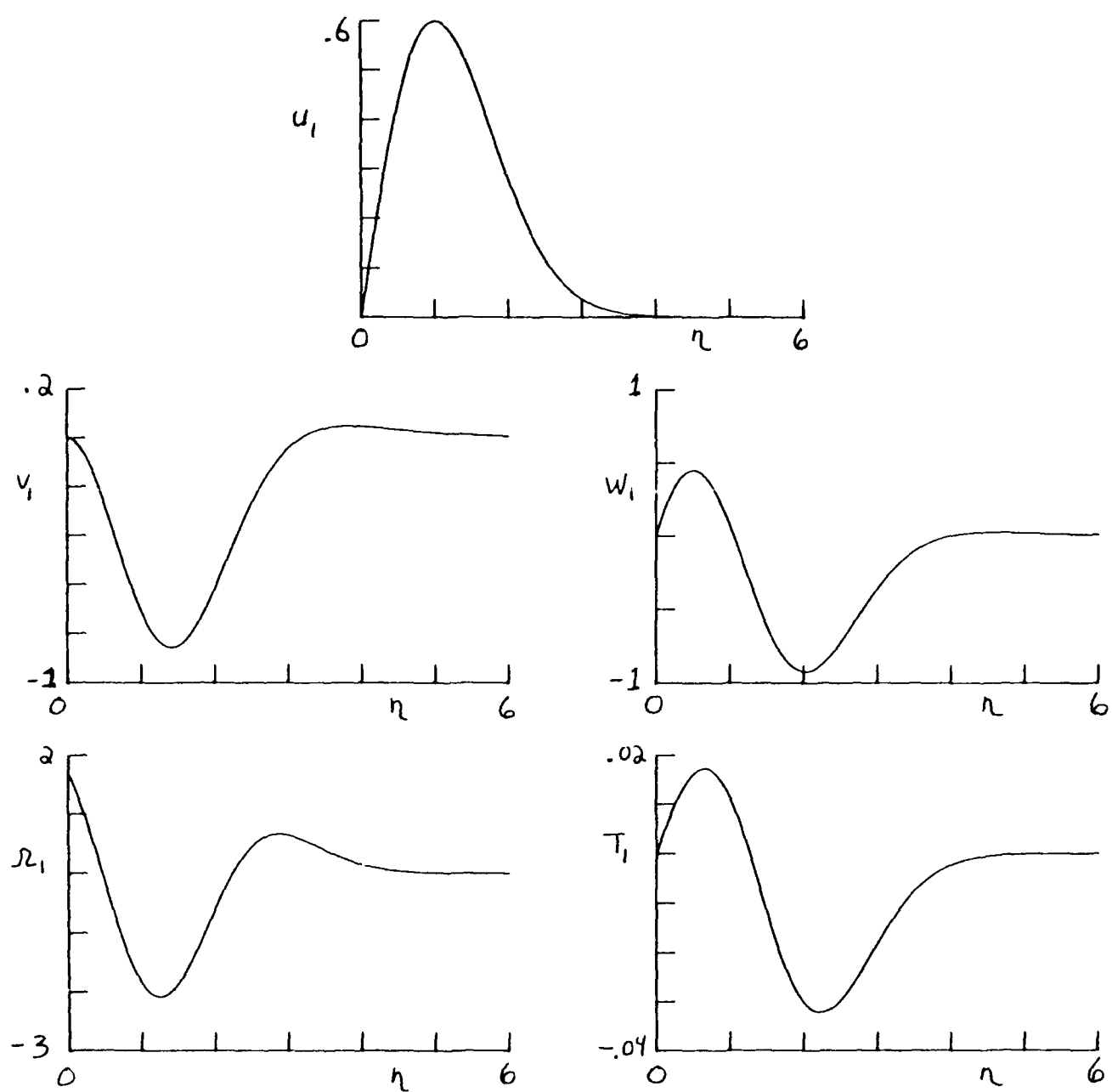
Figure 7c. Eigenfunctions for the third eigenvalue for T_p = 0.8 , \alpha = 0.9 , and \omega = -3.629022 .
