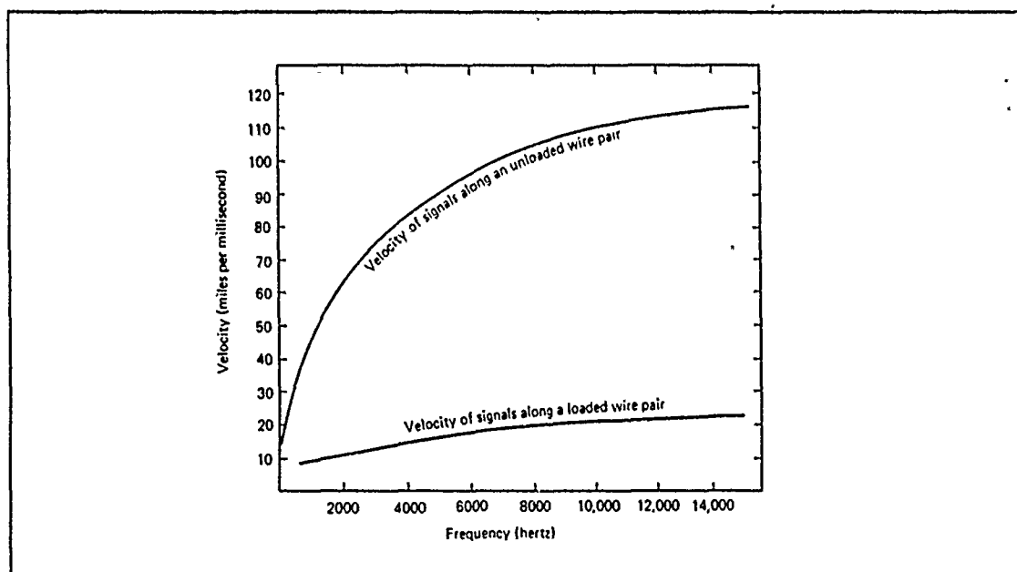
Figure 24. Effect of Loading Coils on Delay Distortion [Ref. 25: p. 165]
