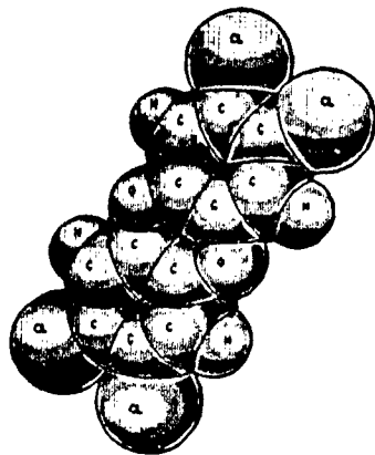
2,3,7,8 - TCDD mw = 321.97
