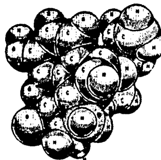
Naloxone mw = 327.37
