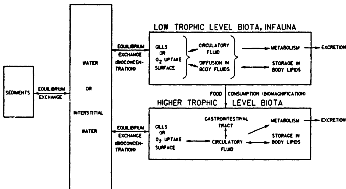
Figure 3. Diagram of routes of uptake and clearance of lipophilic chemicals by aquatic biota (reprinted with permission from Connell 1990)
