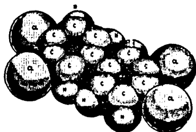
3,3',4,4' - Tetrachlorobiphenyl mw = 292.0
