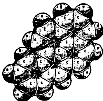
Benzo[a]pyrene mw = 252.3
