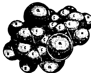
2,2',6,6' - Tetrachlorobiphenyl mw = 292.0
