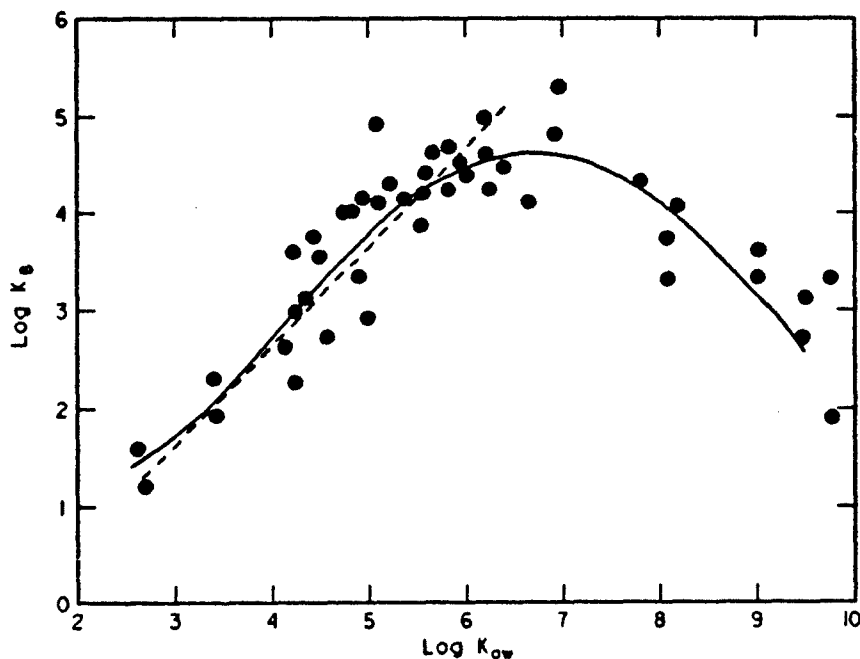
Figure 5. Relationship between \log K_b and \log K_{ow} for bioconcentration (reprinted with permission from Connell 1990)
