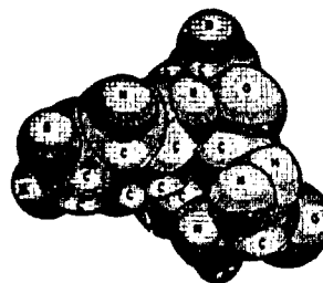
Phenobarbital mw = 232.2
