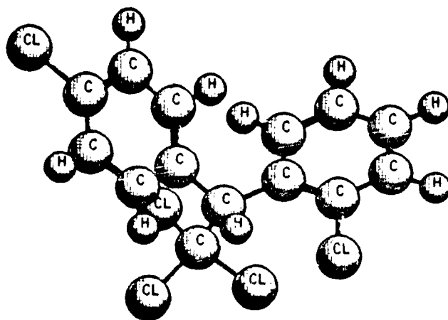
Figure 6. Examples of neutral organic chemicals showing the relationship among size (molecular weight, mw), hydrophobicity (log K_{ow} ), solubility(s), and bioconcentration factor ( K_b )
