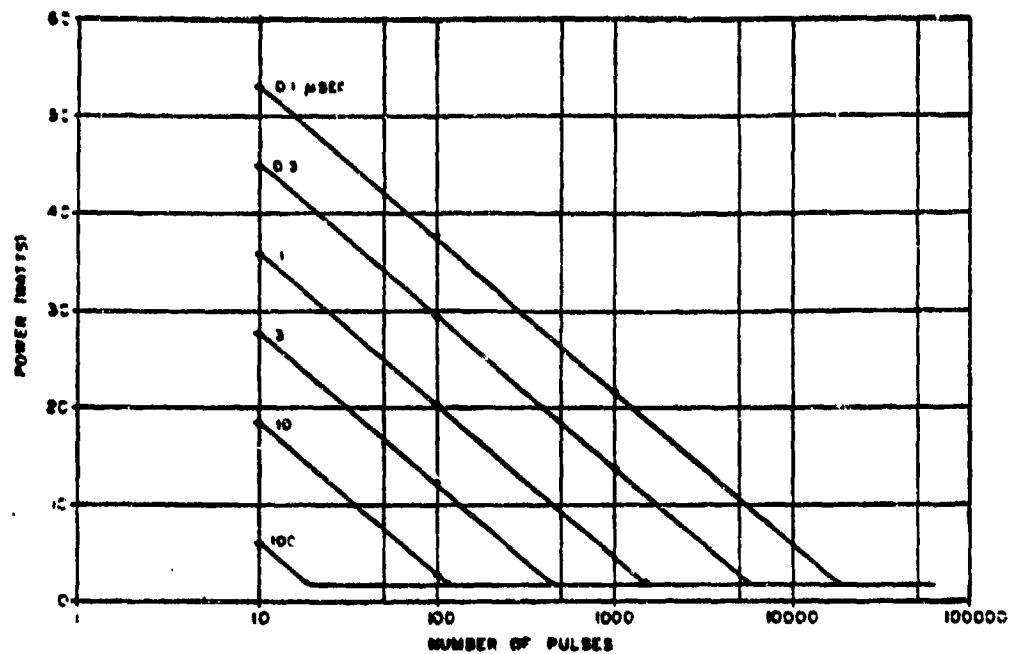
Figure E-44. Peak Absorbed Power for 1N23 Diode 50-Percent Failure Level vs Number of Applied Pulses for Various Pulse Widths. [E-19]
