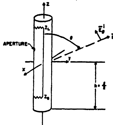
Figure C-7. Cylindrical Enclosure Model. [C-24]
