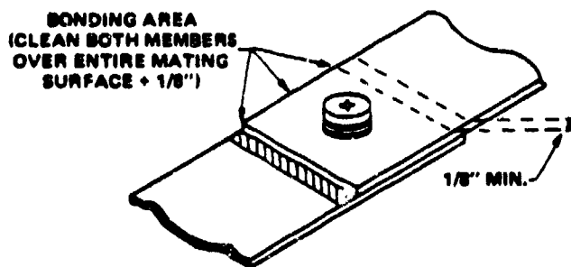
(f) BRACKET INSTALLATION (Rivet or Weld)
