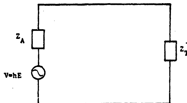
Figure C-12. Equivalent Circuit for Dipole Model.
