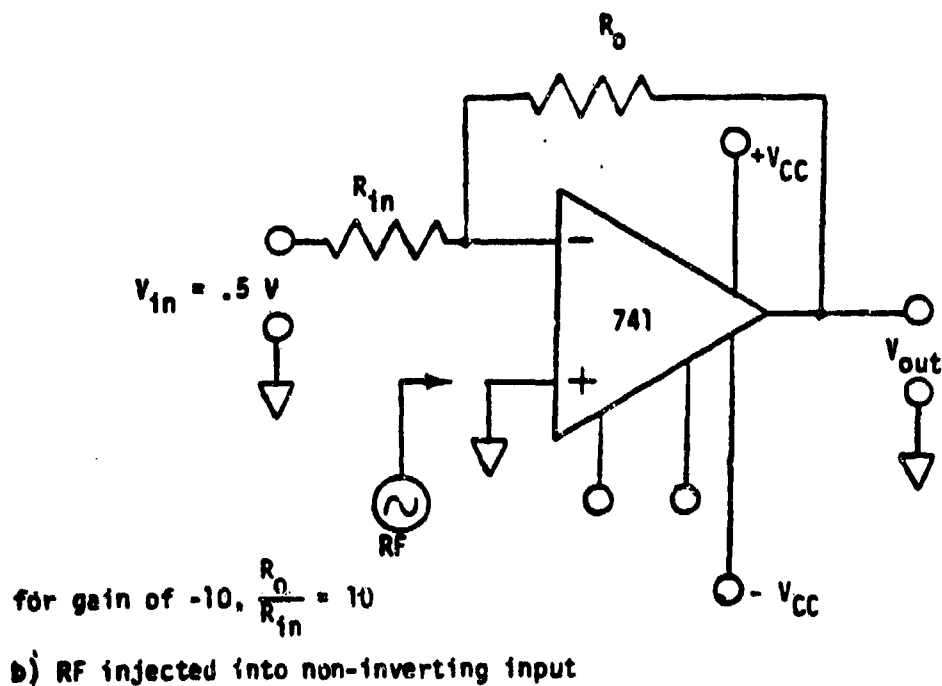
Figure E-12. Test Configurations for 741 Pulsed Interference Tests. [E-12]
