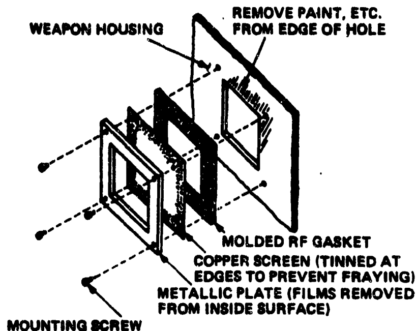
Figure G-6. Method of Mounting Wire Screen Over a Large Aperture. [G-1]
