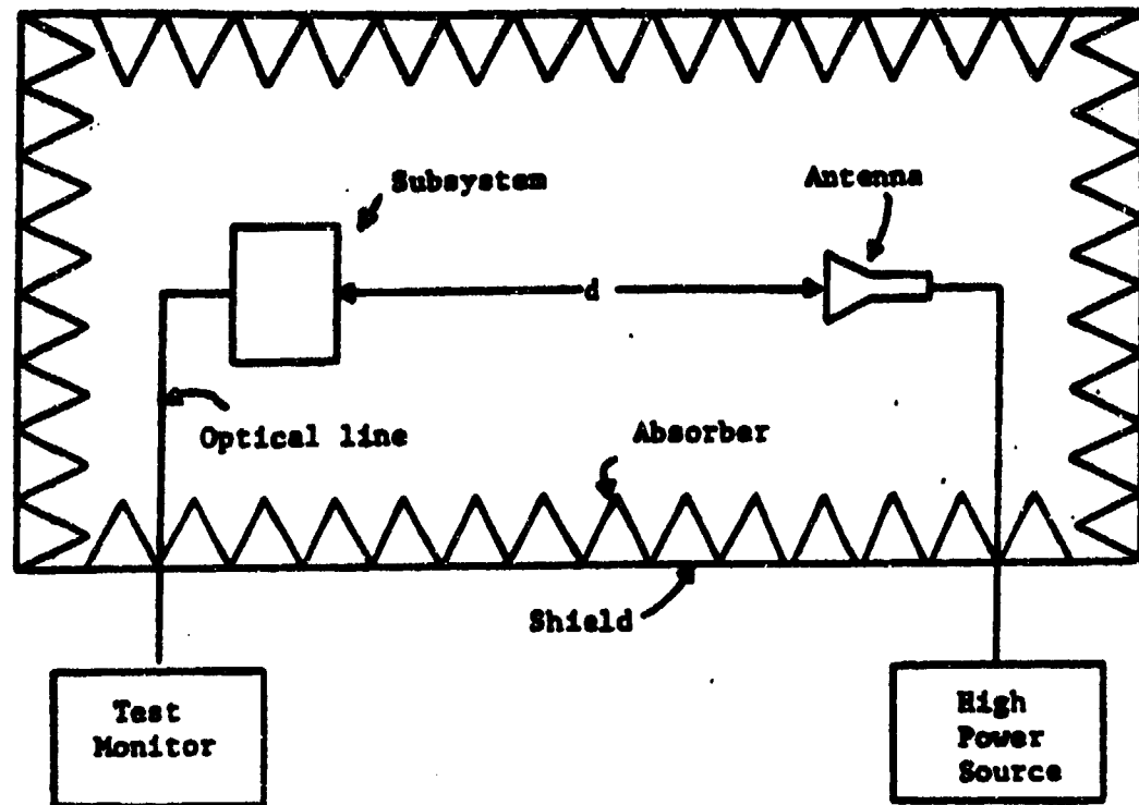
Figure H-13. Radiation Testing in a Chamber Facility.
