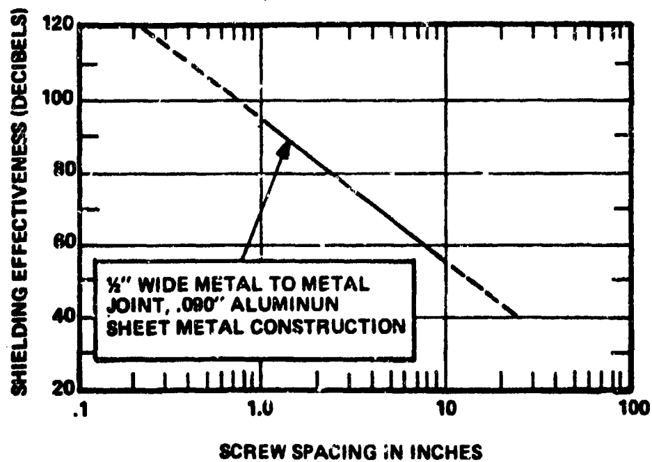
Figure G-19. Influence of Screw Spacing. [G-1]
