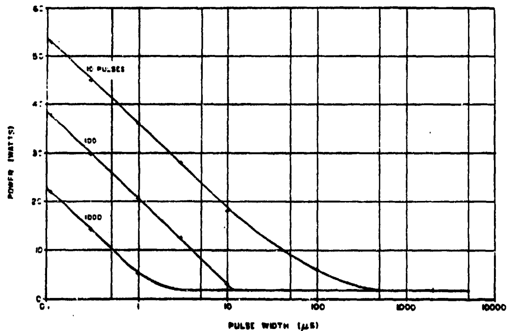
Figure E-45. Peak Absorbed Power for 1N23 Diode 50-Percent Failure Level vs Pulse Width for Various Numbers of Applied Pulses. [E-19]
