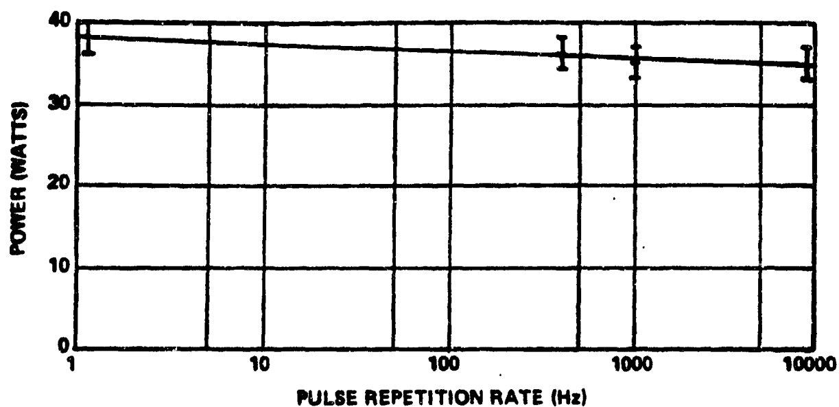
Figure E-43. Peak Absorbed Power Required for 1N23 Diode 50-Percent Failure for 1\mu\text{S} Pulse Width. [E-19]
