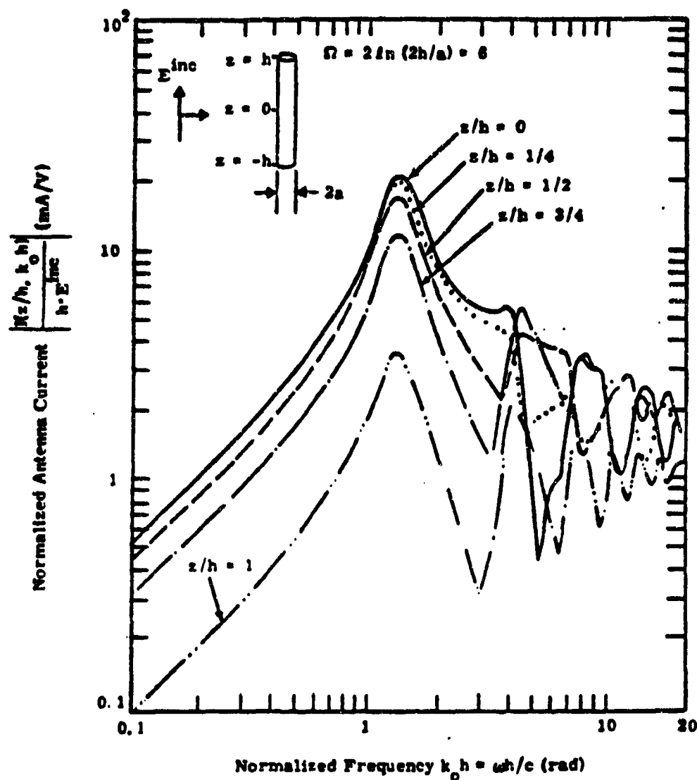
Figure C-16. Transfer Function for Total Axial Current on a Cylinder with Endcaps. [C-2]
