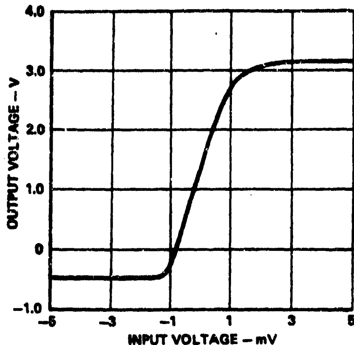
Figure E-22. Typical Voltage-Transfer Curve for Type 710 Comparators. [E-13]
