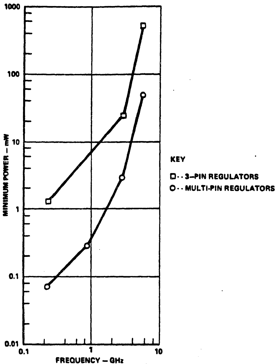
Figure E-20. Composite Worst-Case Susceptibility Values for Voltage Regulators. Output Voltage Change of 0.25 Volt is Susceptibility Criterion. [E-13]
