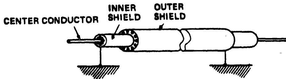
Figure G-21. Examples of Grounding A Double-Shielded Coaxial Cable. [G-1]
