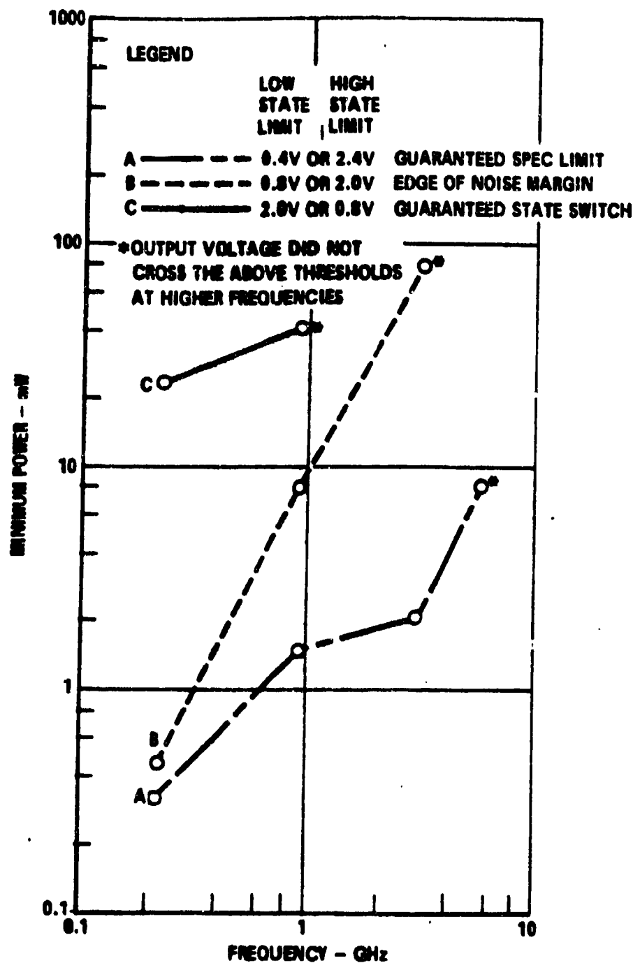
Figure E-24. Composite Worst-Case Susceptibility Values for TTL Devices. [E-13]
