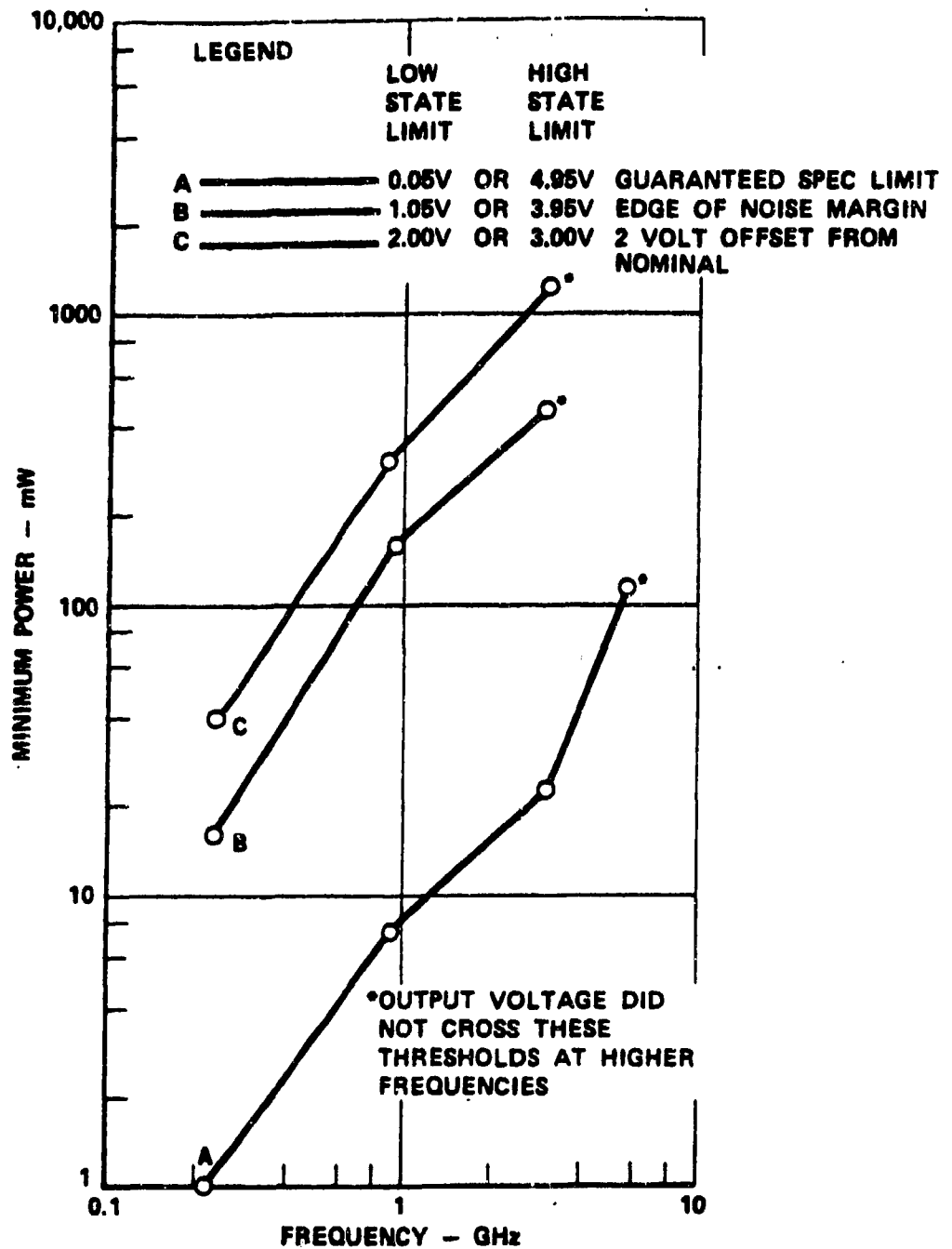
Figure E-25. Composite Worst-Case Susceptibility Values for CMOS Devices. [E-13]
