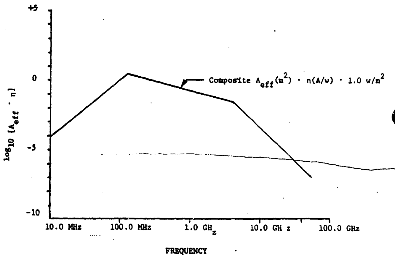
Figure C-24. Composite curve of Coupled Power and Component Response. [C-24]
