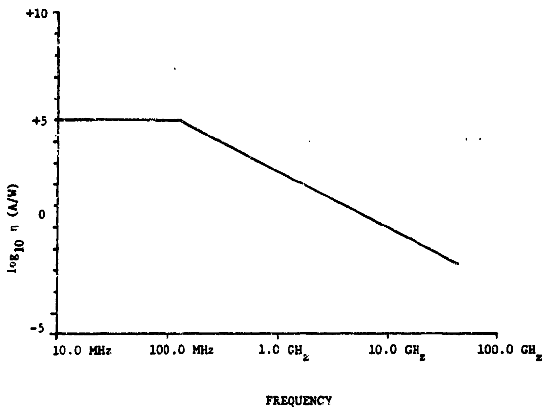
Figure C-23. Maximum Rectification Efficiency of a Component. [C-24]
