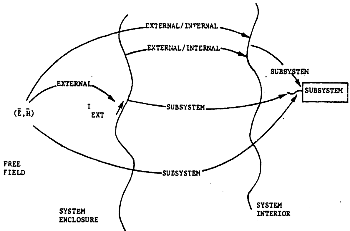
Figure C-29. General Coupling Modes. [C-55]
