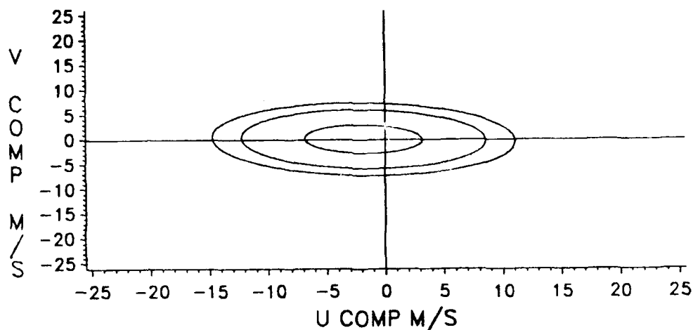
Figure E-42. Wind Probability Ellipses, January, 20 KM.
