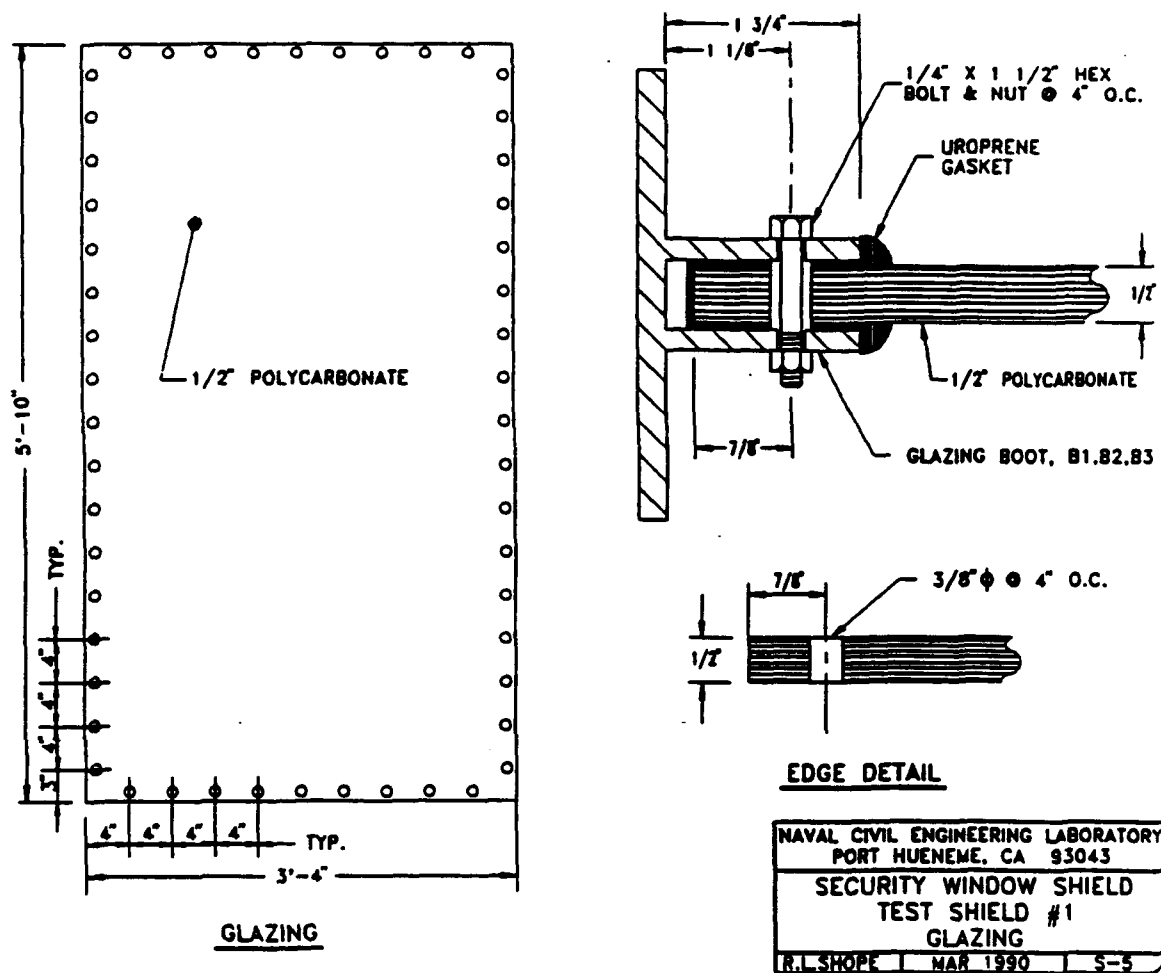
Figure 4-13. Prototype design - polycarbonate glazing.
