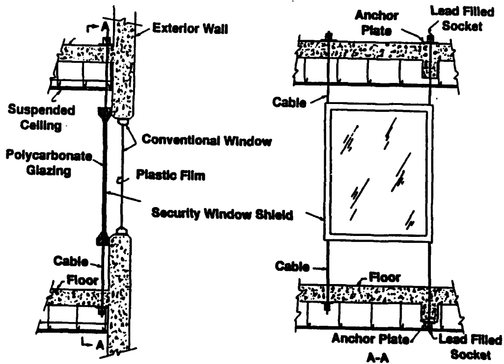
Figure 2-8. Safety window shield installed in reinforced concrete building.
