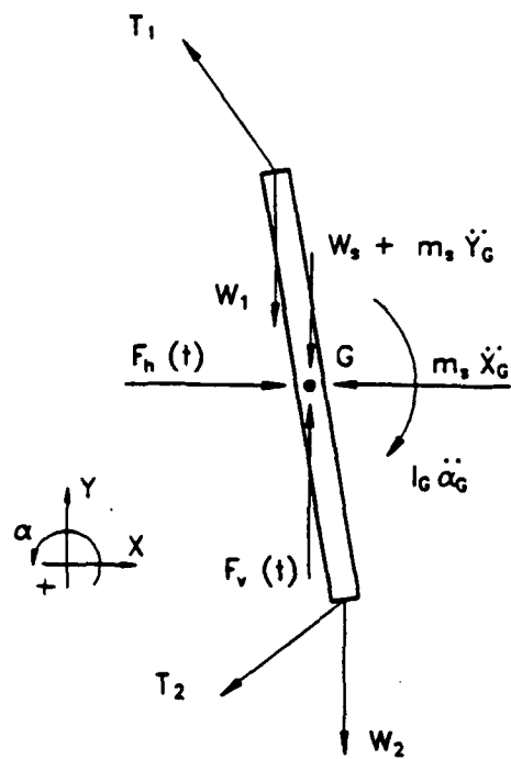
Figure 3-3. Free body diagram of shield.
