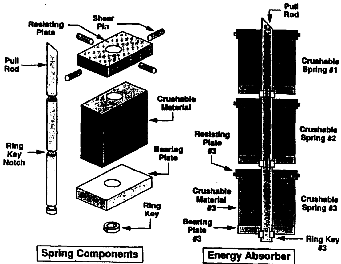
Figure 2-3. Energy absorber components.
