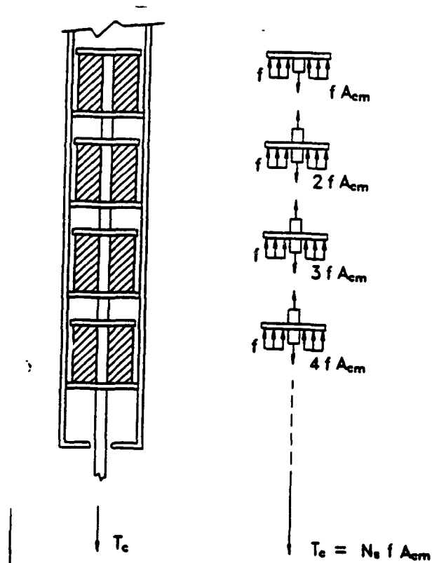
Figure 3-4. Forces applied to energy absorber.
