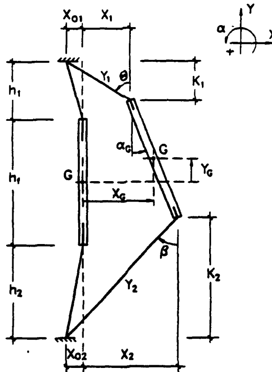
Figure 3-2. Definition of geometric parameters for displaced shield.
