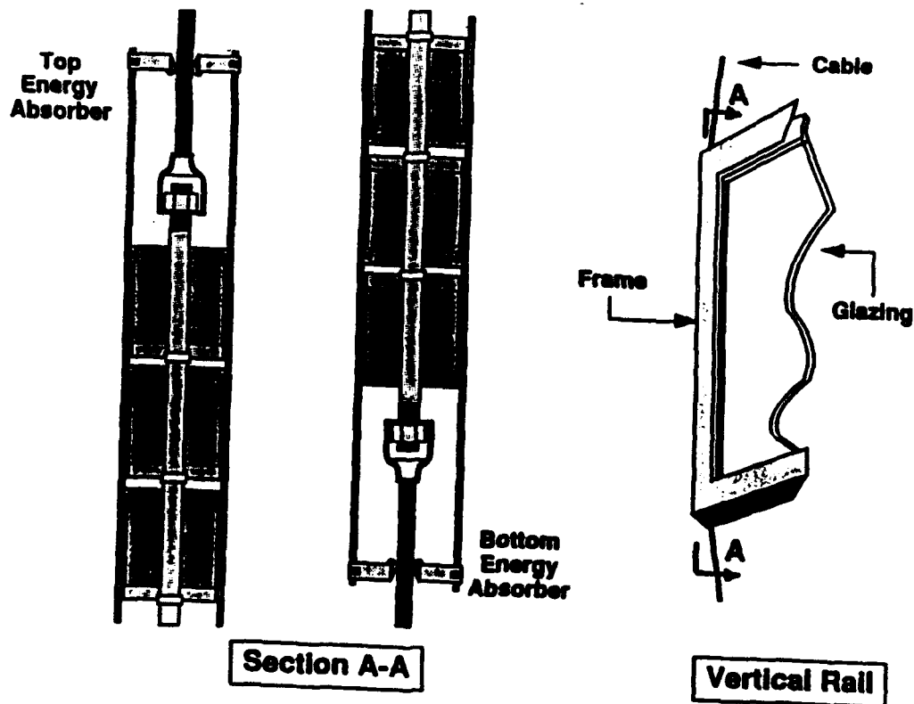
Figure 2-2. Cables and energy absorbers.
