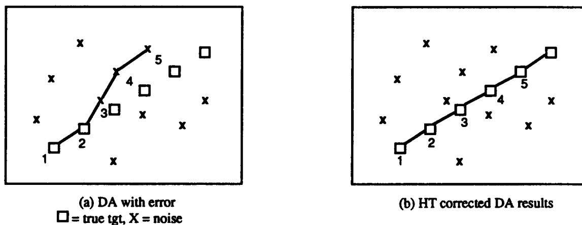
Figure 5: DA error corrected by HT peak mismatch
