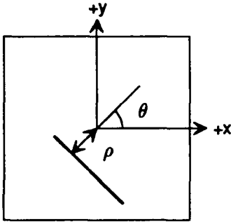
Figure 1: Straight line in input space and its corresponding Hough space parameters \rho and \theta .
