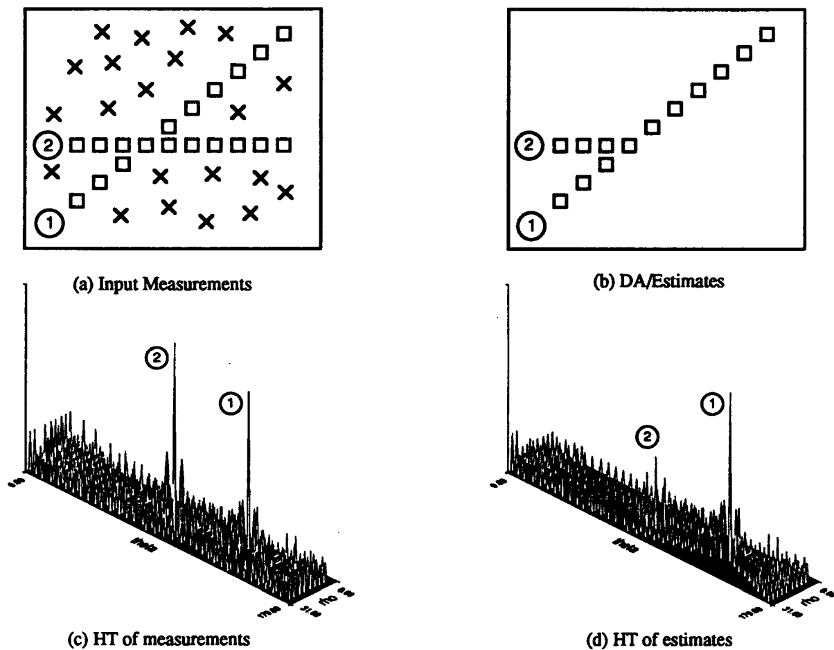
Figure 4: HT with merged measurement DA error
