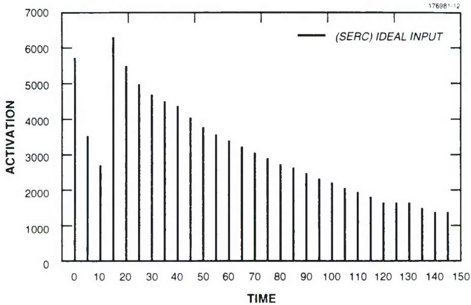
Figure 15. SERC ideal input source function. Converged (fourth generation) for spatial separation of nine nodes between inputs with an ISI of 150 time units.
