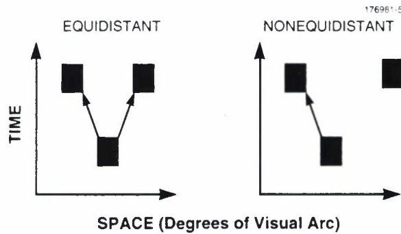
Figure 6. Split effects. Illuminating one point source followed by illuminating two equidistant point sources cause the first to appear to split and move to both of the later sources. If these are not equidistant to the first, movement is only to the closer of the pair.
