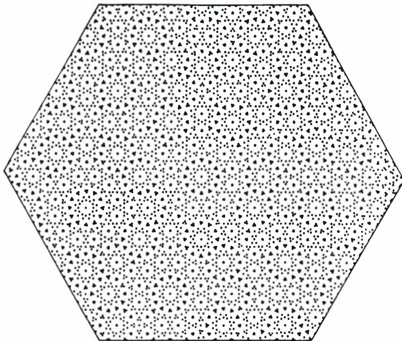
Figure 1. Static feature grouping on multiple scales: evidence for the existence of a grouping process in the visual system [8].
