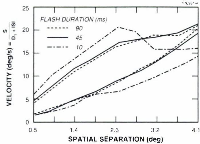
Figure 5. Calculated velocity versus spatial separation [1].
