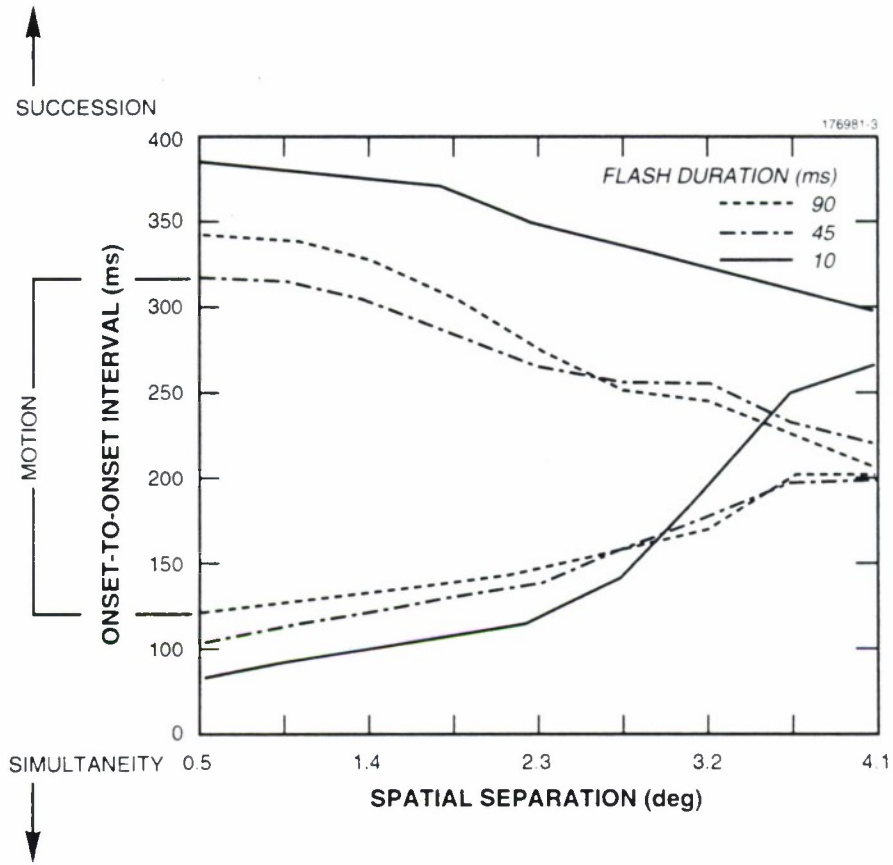
Figure 4. Parameters affecting long-range apparent motion. SOA versus spatial separation [1].
