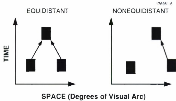
Figure 7. Merge effects. Illuminating two point sources equidistant from a third, later-illuminated point source gives the appearance of the two merging and becoming one. If the original pair is not equidistant from the third point source, only the closer of the two will appear to move.
