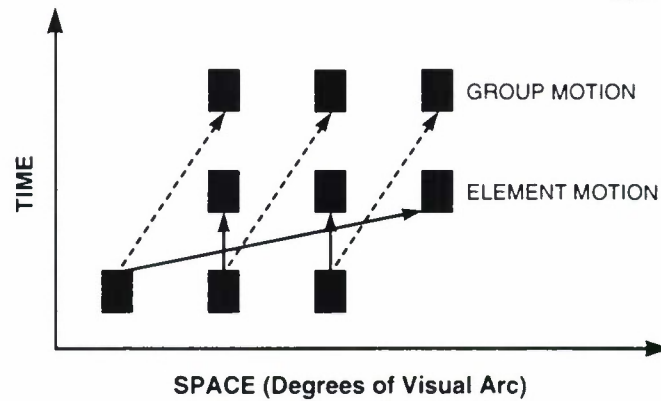
Figure 8. Ternus effect. Illuminating shifting groups of three point sources produces the illusion of one in element motion or all three in group motion. The percept changes with changing ISI.
