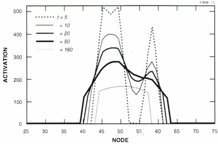
Figure 16. Multiscale grouping. Three inputs at nodes 45, 49, and 58 interact on increasing scale with increasing time. Discrete activation on the CE layer is pictured as continuous curves.
