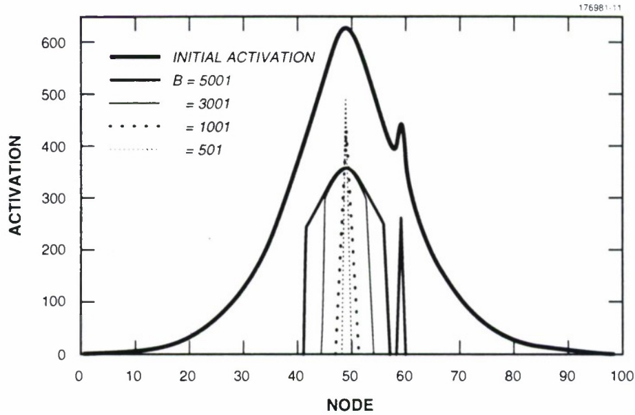
Figure 14. Feedback activation profiles. As B decreases so does the extent of the feedback until the network selects only the maximum node. By causing B to decay between inputs, the network forgets earlier stimulation and reproduces the extinguishing half of the gamma effect.
