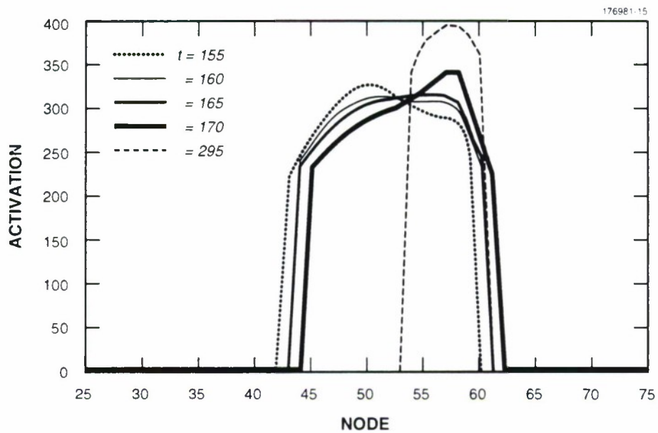
Figure 18. Long-range apparent motion between two inputs. The maximum of activity on the CE layer moves between the initial source located at node 50 and the final source located at node 59, generating the appearance of long-range motion. Discrete activation on the CE layer is pictured as continuous curves. In this case, the maximum of activity exhibits a jump, as in Figure 3.
