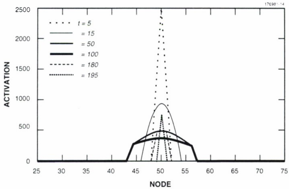
Figure 17. Gamma effect. A single input initially induces a narrow maximum, which expands, stabilizes, and extinguishes after the input is turned off at t = 150 . Discrete activation on the CE layer is pictured as continuous curves.
