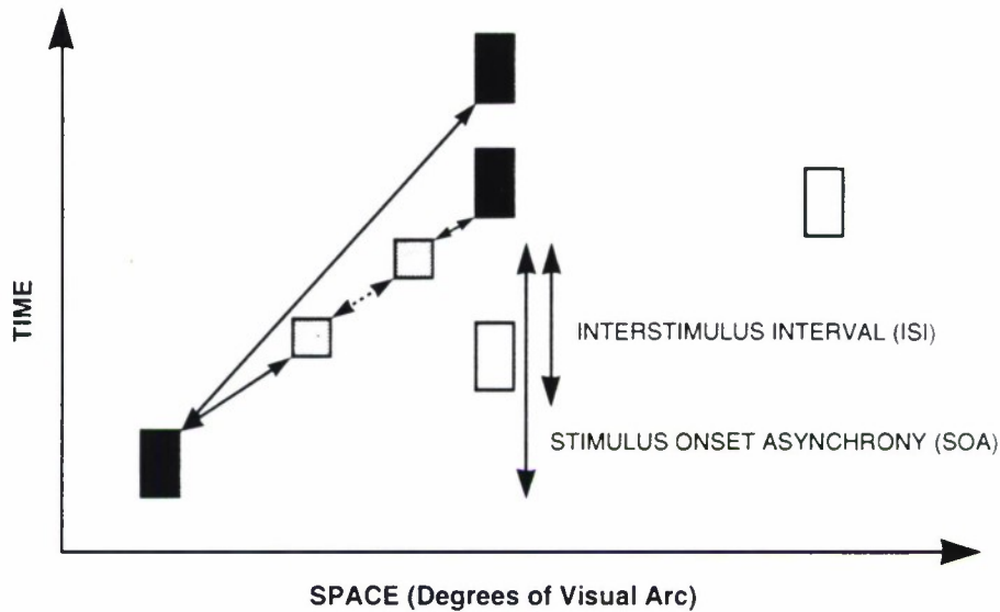
Figure 3. Long-range apparent motion. The filled rectangles represent sources in space-time separations that produce the illusion of long-range apparent motion. The empty rectangles represent sources that are ignited too soon for the spatial distance or are too far away for the given ISI. The center rectangle occurs soon enough to give the appearance of smooth motion from the left-most rectangle to the first shaded square, a short jump to the second shaded square, followed by smooth motion to the destination, while the upper rectangle exhibits pure smooth motion.
