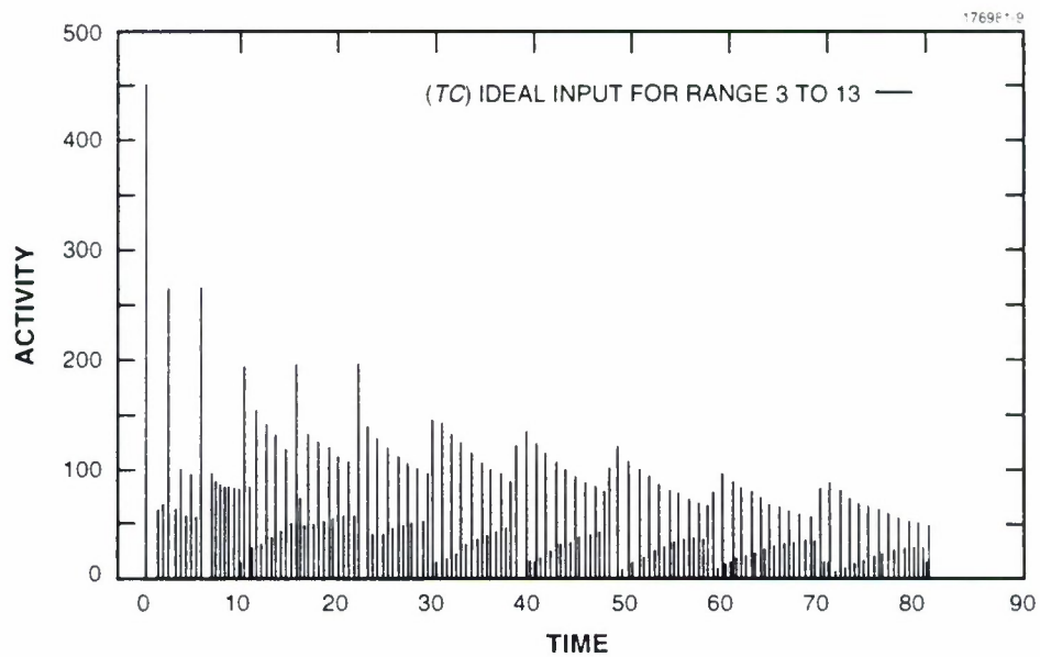
Figure 12. TC ideal input. The scalloped effects are due to each smaller displacement arriving at its final destination.
