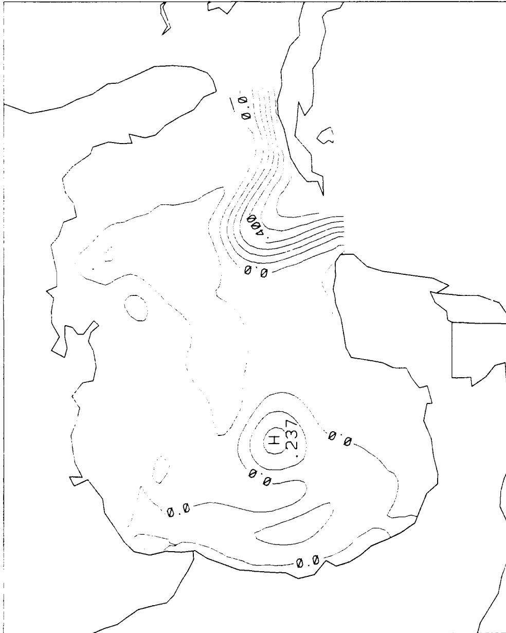
Fig. 2b: Sea Surface Height contours for simulated observations, Case A: \beta_0 = 0.10 , \beta_1 = 1.00
