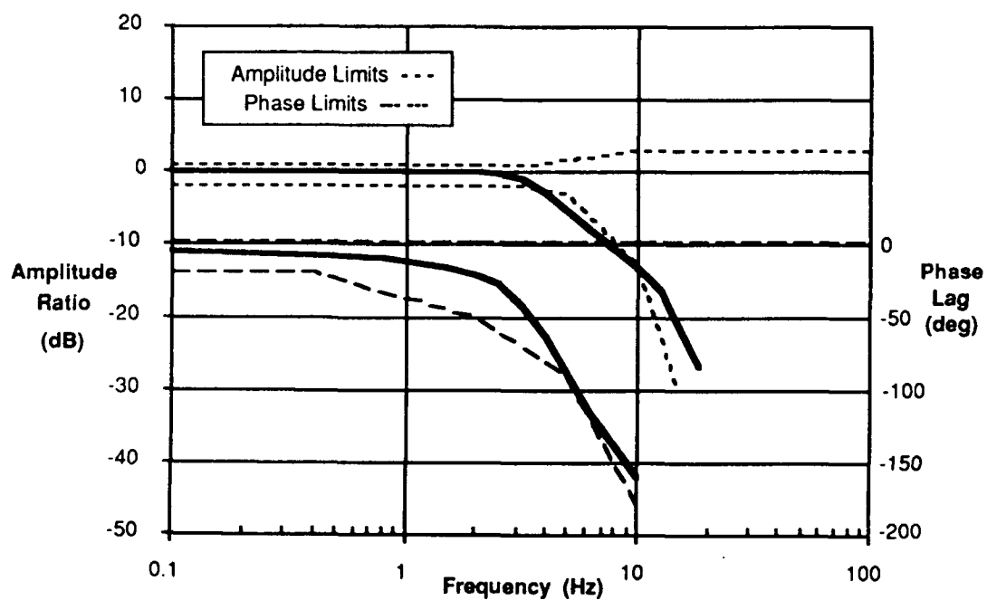
Figure 76. Divergent Flap Frequency Response 10% Amplitude
