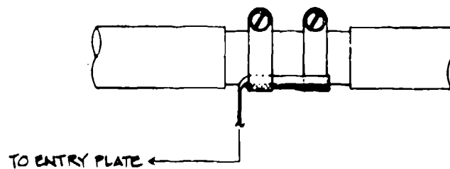
Figure 1-33. Grounding Steps for Cables
