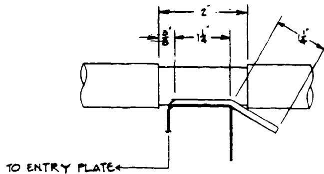
Figure 1-32. Ground Strap Detail
