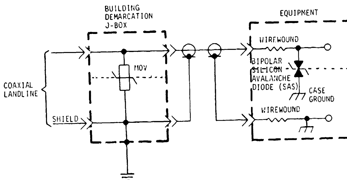
a. TYPICAL TRANSIENT PROTECTION CONFIGURATION
