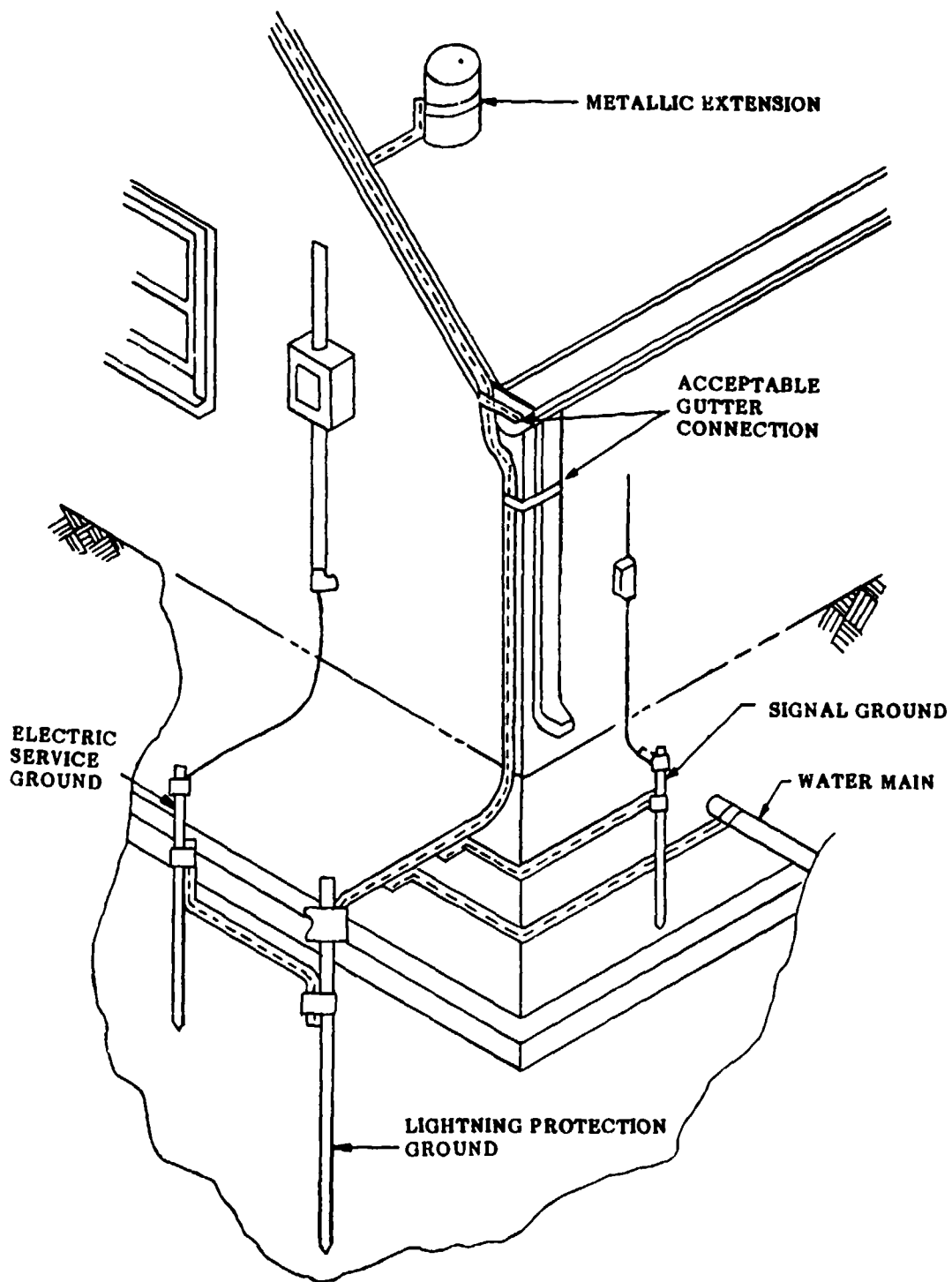
Figure 1-15. Grounding Practices for Lightning Protection
