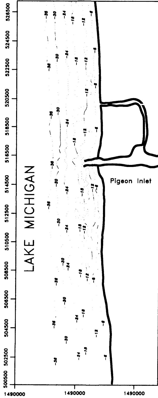
Figure 8. Hydrographic survey of Port Sheldon, Michigan, and vicinity, 1965
