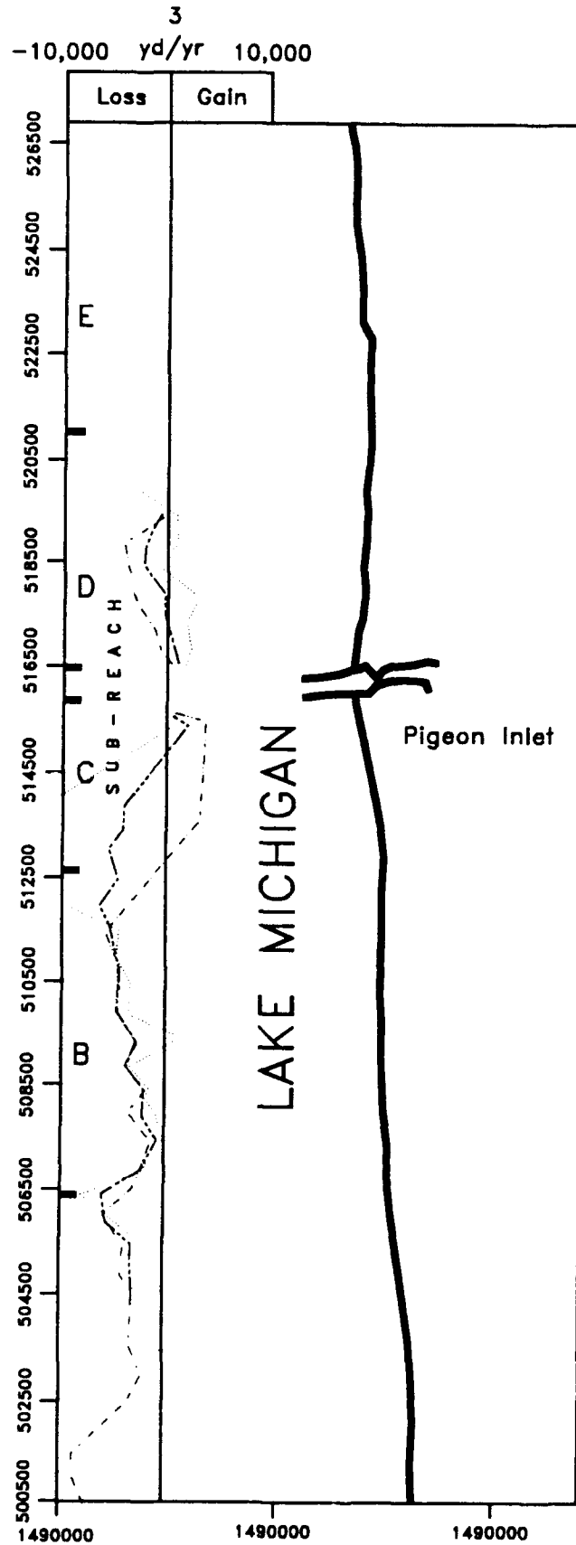
Figure 10. Rates of volumetric change (cubic yards/year) plotted with 1984 shoreline
