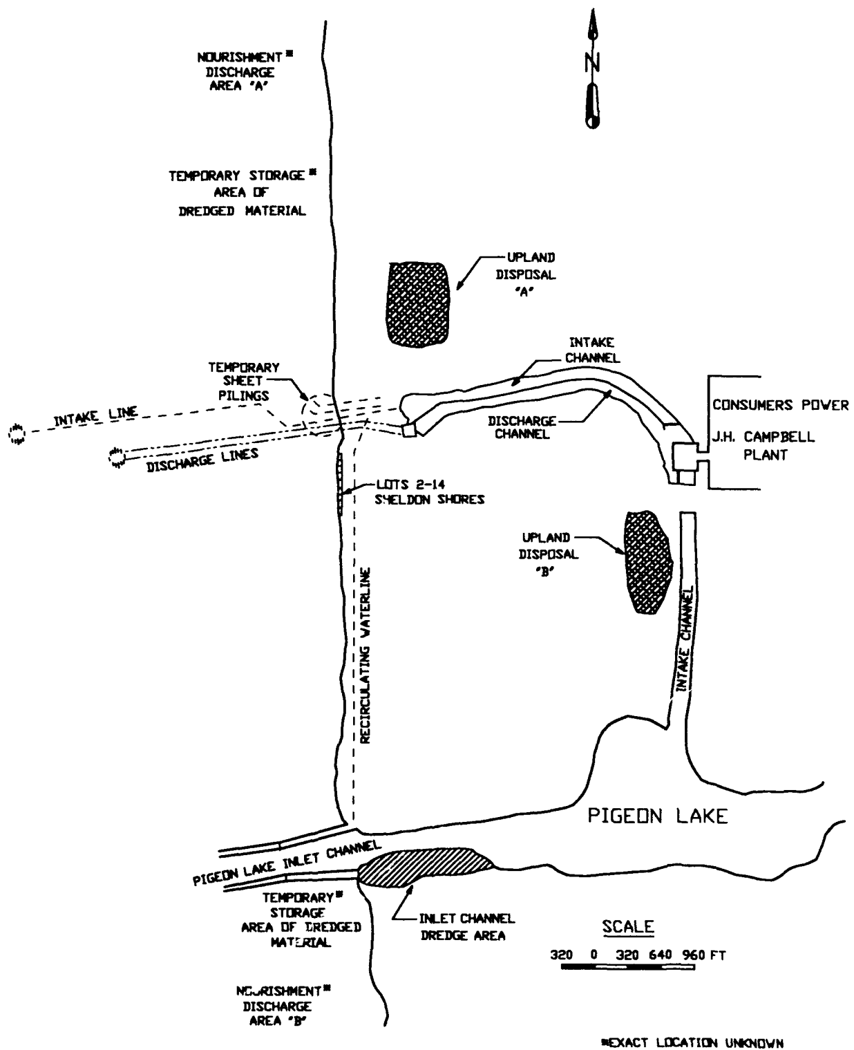
Figure 2. Schematic of the Port Sheldon area with dredge disposal sites
