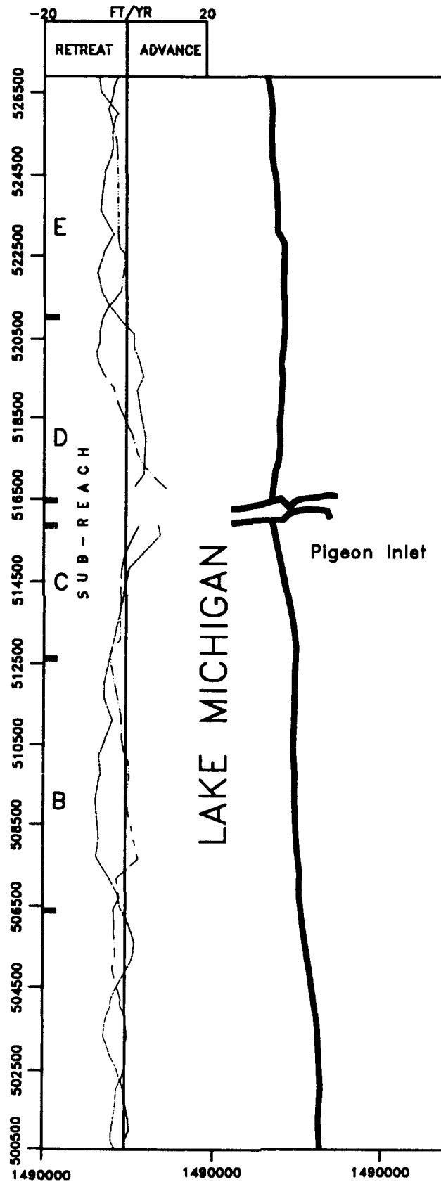
Figure 6. Rates of shoreline change (feet/year) plotted with 1984 shoreline
