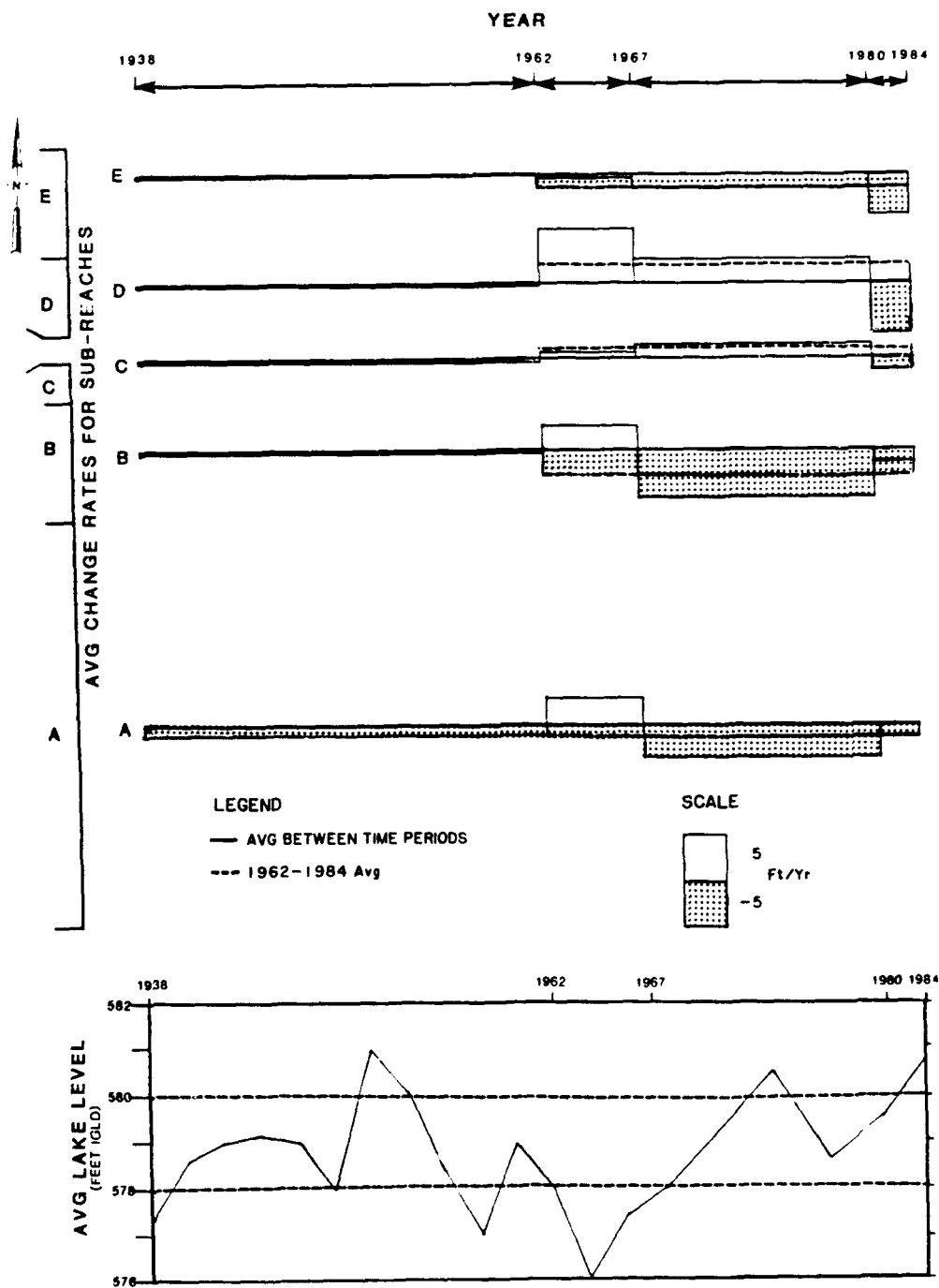
Figure 4. Average change rates for subreaches between time periods with corresponding Lake Michigan average lake levels
