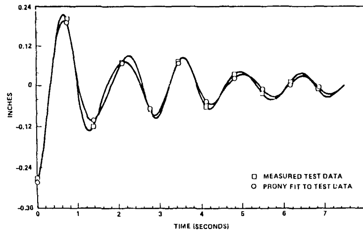
Initial NASTRAN Model Versus Prony Fit
