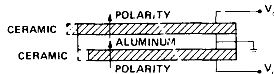
PUSH-PULL BENDING ACTUATOR
