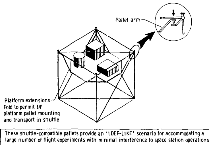
Fig. 9. Cargo bay size equipment pallets can be recessed in 5-meter truss to minimize station congestion.
