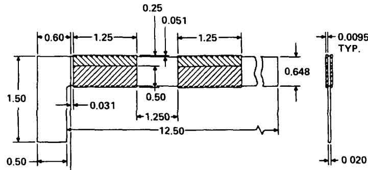
ACTUATOR/SENSOR LOCATIONS FOR MIMO PIEZOBREAM. ALL DIMENSIONS IN INCHES.
