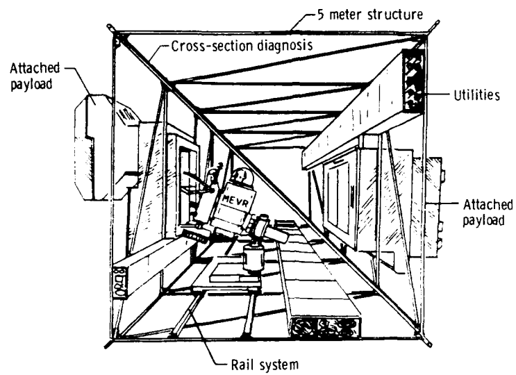
Fig. 14. 5-meter truss provides sufficient room for an interior mobile transporter.
