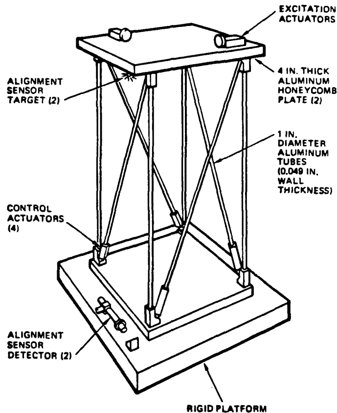
Figure 1: Large Space Structure Truss Experiment Configuration
