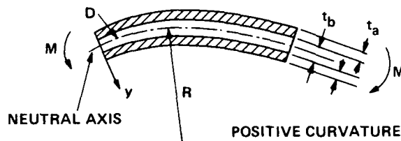
ACTUATOR INDUCED BENDING MOMENT
