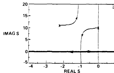
ROOT LOCUS FOR SCALAR PPF
