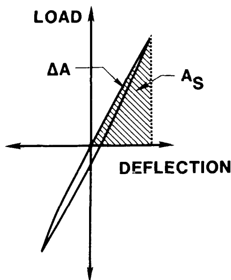
Typical Static Load-Deflection Test Data
