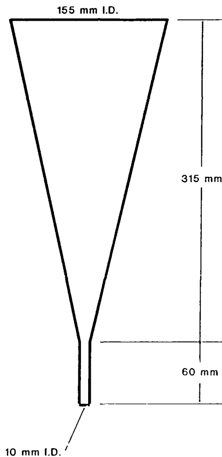
Figure C1. Marsh flow cone
