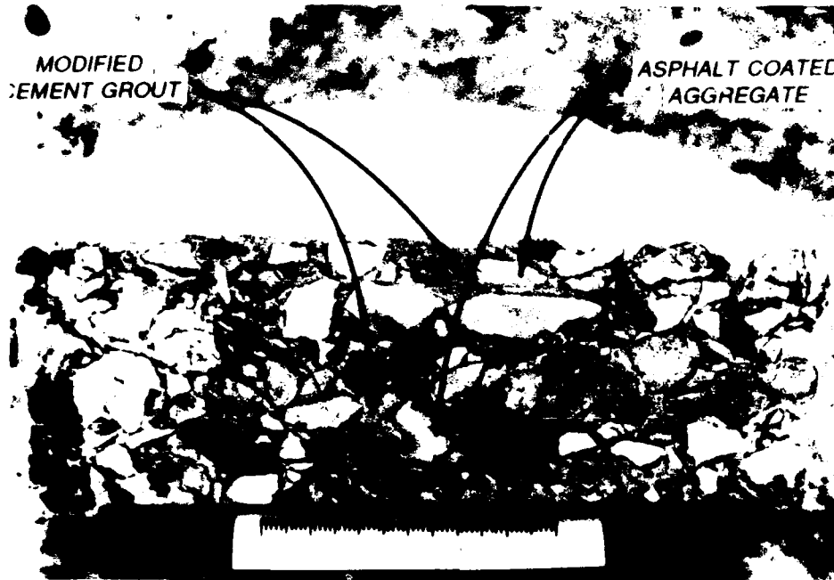
Figure 1. Cross section of RMP specimen
