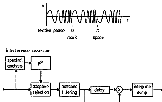
Figure 16 Chirp signal DPSK waveforms and detector.
