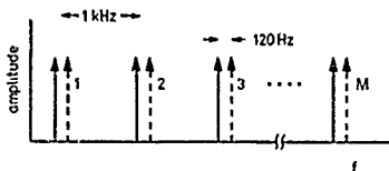
Figure 12 Idealized spectrum for FSK signal with Mth-order frequency diversity. (The mark frequencies are shown by continuous lines, and the space frequencies by broken lines)
