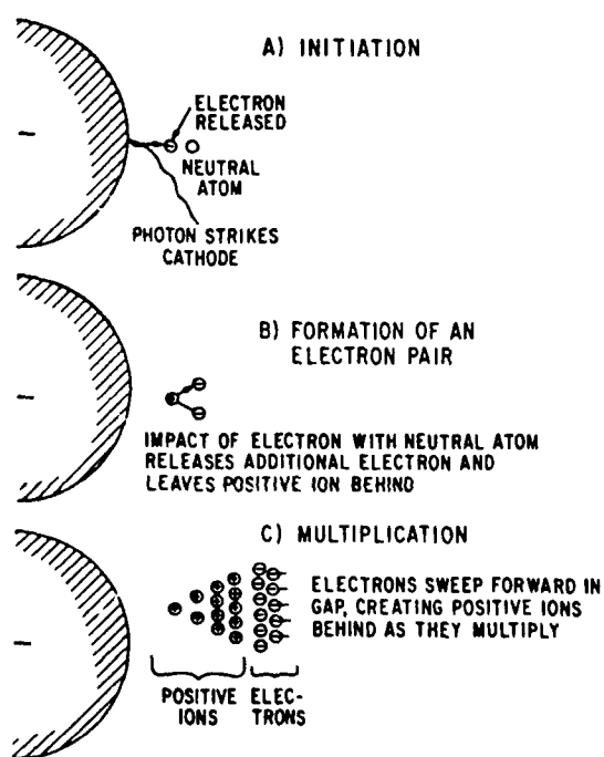
Figure 1. Electron avalanche. Copyright © 1987. Electric Power Research Institute. EPRI EL-2500. Transmission Line Reference Book: 345 KV and Above. Second Edition. Reprinted with permission.
