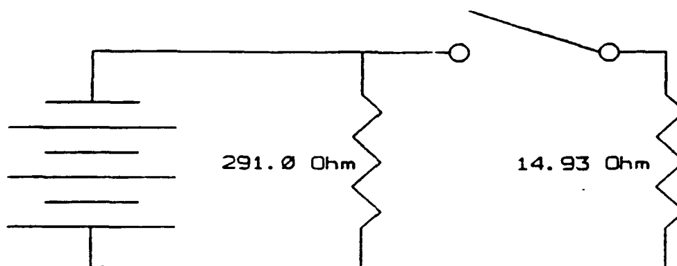
Figure 1. Discharge schematic.
