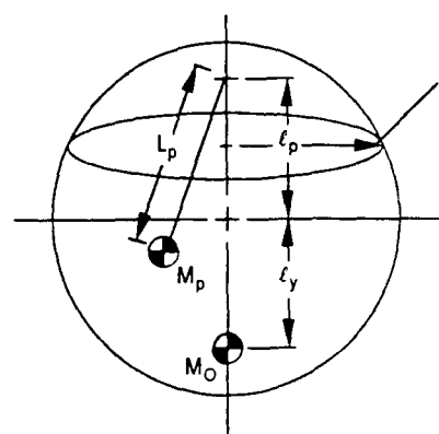
MECHANICAL EQUIVALENT
