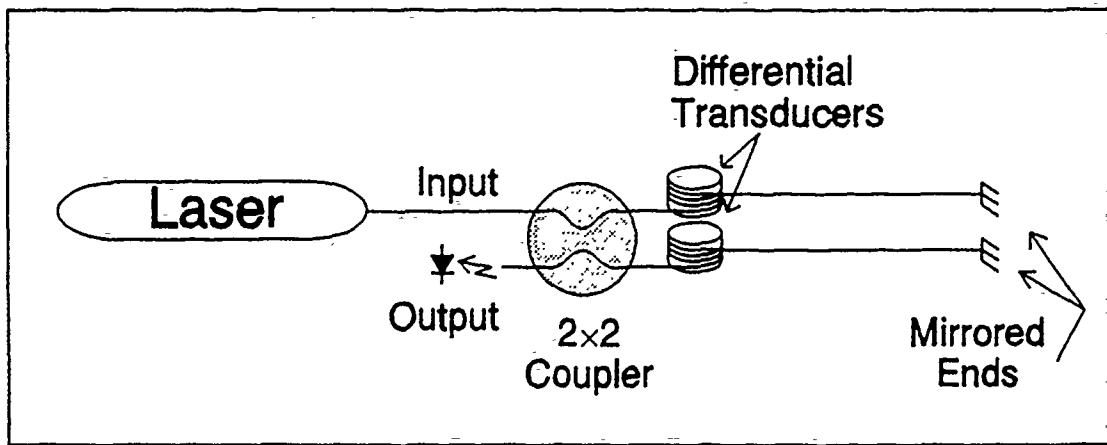
Figure 3 Michelson Optical Fiber Interferometer with a single 2x2 optical fiber coupler for input and output.
