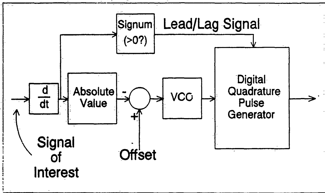
Figure 74 Block diagram of a Digital Quadrature Phase Modulation Simulator.
