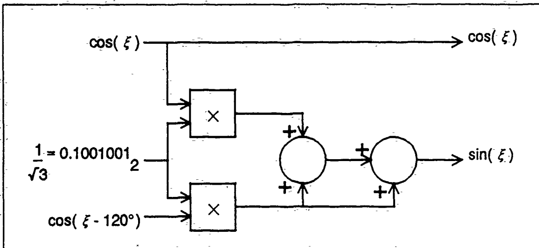
Figure 60 Block diagram showing how to obtain the in-phase and quadrature wave forms without overflow.
