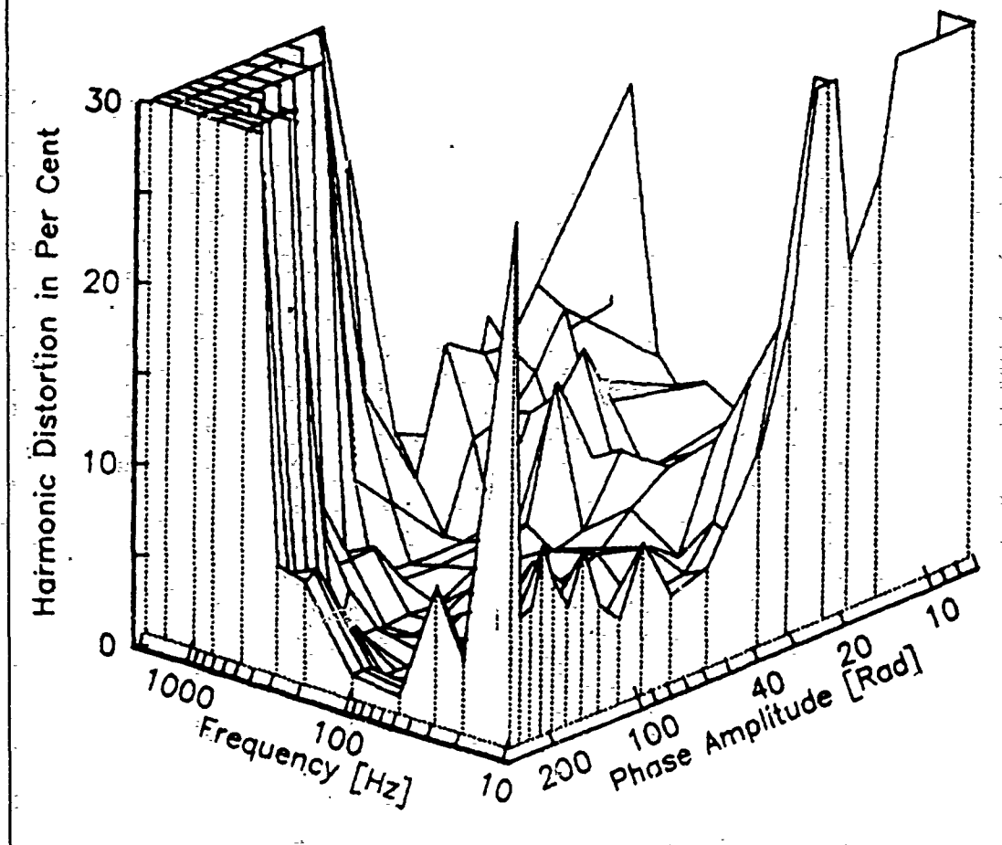
Figure 64 Surface plot showing the total harmonic distortion in the Asymmetric Digital Demodulator as a function of various combinations of input optical phase shift and frequency .
