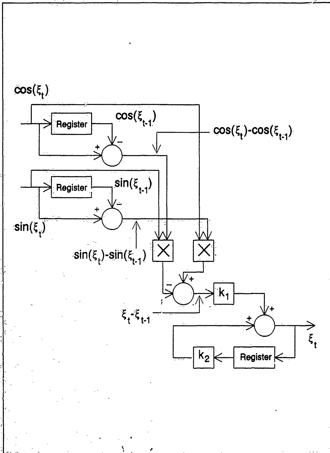
Figure 61 Block diagram showing the asymmetric demodulation algorithm when the data are digital words taken at successive sampling instants t-1, t, t+1, \text{etc.}
