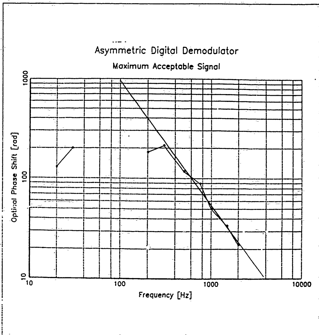
Figure 65 Maximum phase amplitude acceptable to the Asymmetric Digital Demodulator as a function of input frequency. The straight line extrapolates the region of constant phase rate to low frequencies.
