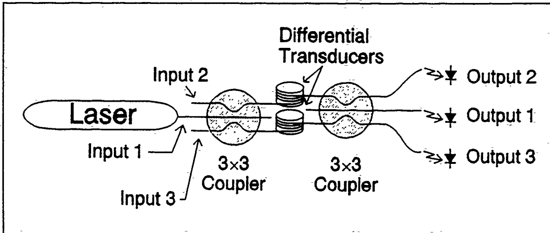
Figure 5 Schematic of a Mach-Zender optical fiber interferometer with a 3×3 coupler at the input and a 3×3 coupler at the output.
