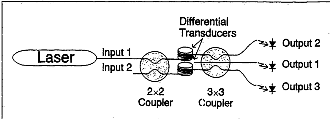
Figure 4 Schematic of a Mach-Zender optical fiber interferometer with a 2×2 coupler at the input and a 3×3 coupler at the output.
