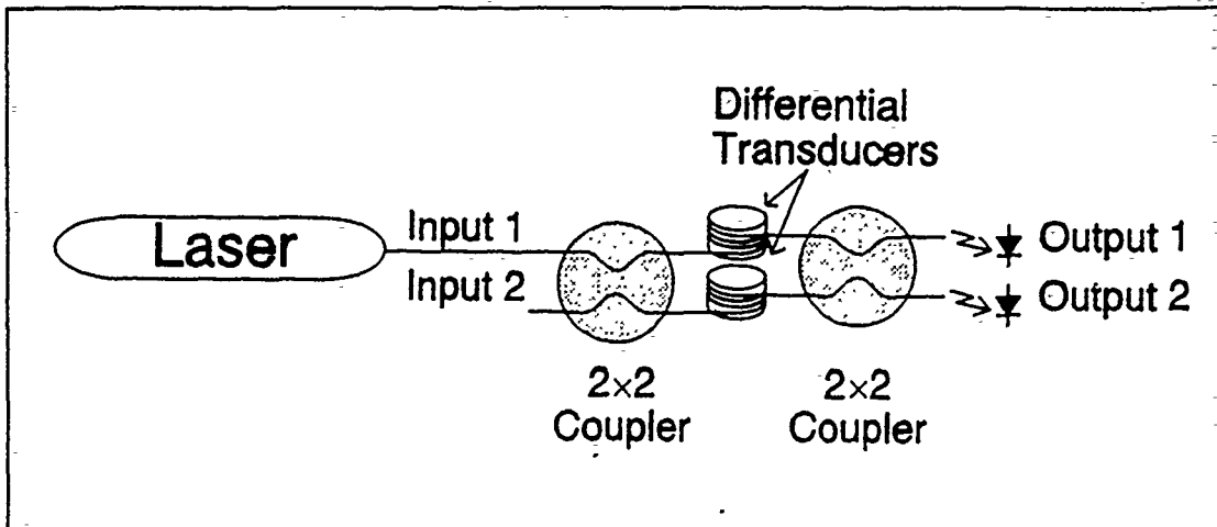
Figure 2 Mach-Zender Optical Fiber Interferometer with 2x2-optical fiber couplers at input and output.
