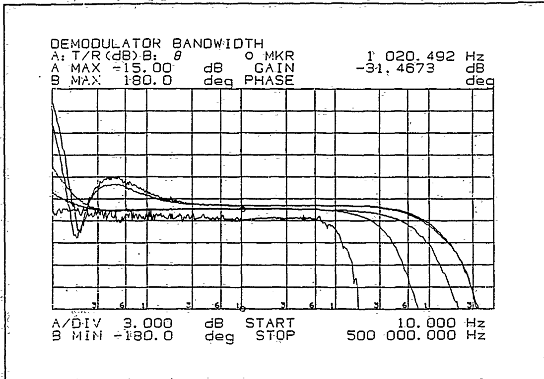
Figure 47 Measured bandwidth of the Symmetric Analog Demodulator (113 kHz for small signals). In descending order of bandwidth, the phase inputs to the demodulator were 219 mrad, 690 mrad, 2.17 rad, 5.54 rad, and 9.28 rad.
