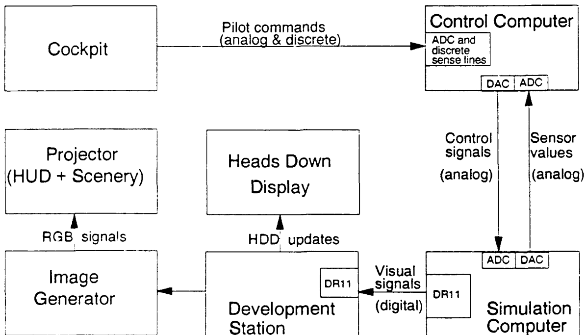
Figure 2. System Communications
