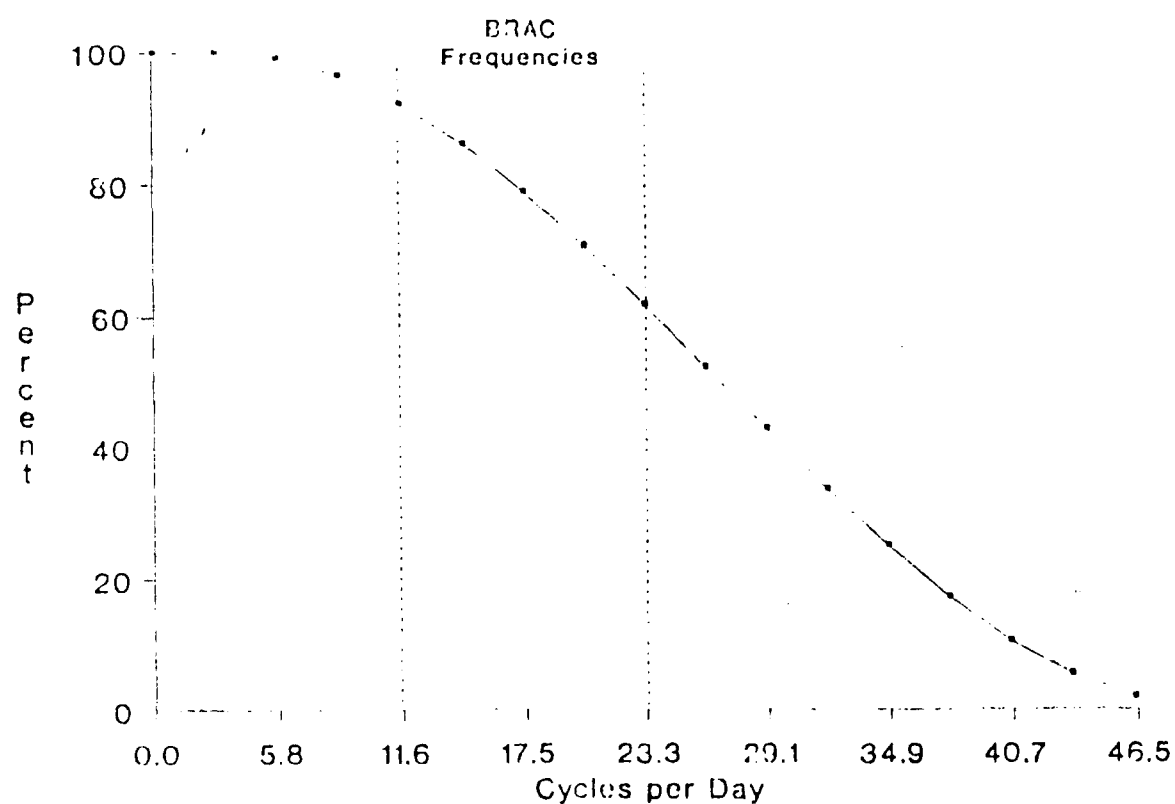
Figure 8 - Filter frequency response function
