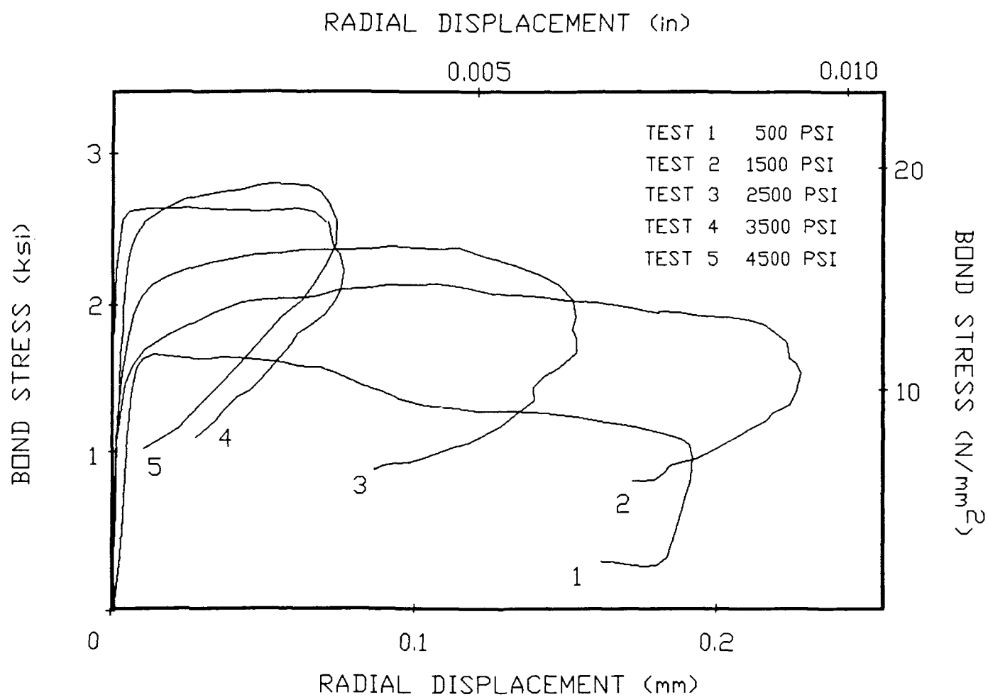
Figure 14. Tests 1 through 5: Radial displacement histories.
