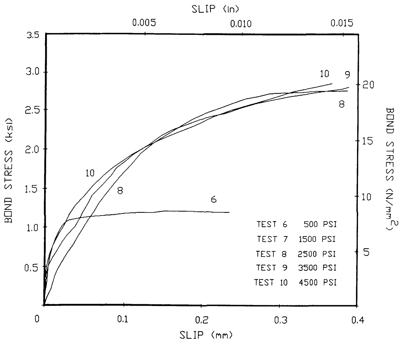
Figure 18. Tests 6 through 10: Initial post-cracking bond-slip.
