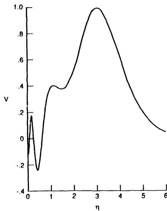
Figure 4c. Eigenfunction of the fourth mode for a Mach number of 5 and a = 1.25 .
