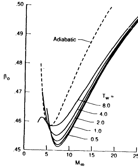
Figure 12. The neutral growth rate \beta_0 from (6.3) for the trapped layer modes as a function of M_\infty for an adiabatic fluid and also for an isothermal fluid with T_w = 0.5, 1, 2, 4, 8 .
