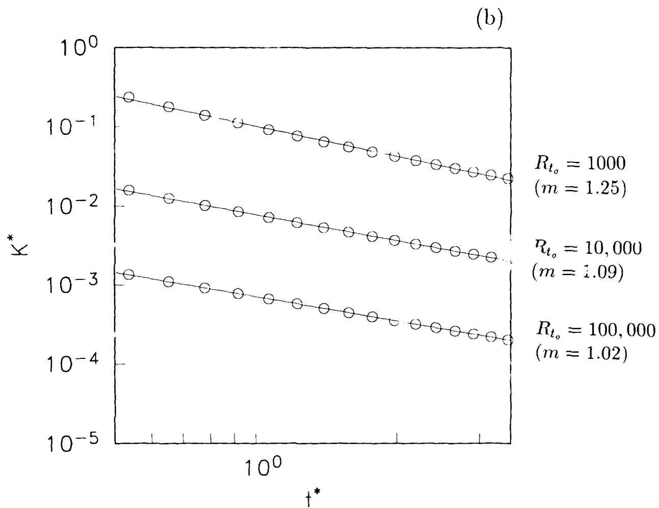
Figure 10. Decay of turbulent kinetic energy: \circ Self-preserving solution; — K \propto t^{-m} . (a) C_{\epsilon_2} = 4 , (b) C_{\epsilon_2} = 4.5 , and (c) C_{\epsilon_2} = 5 .
