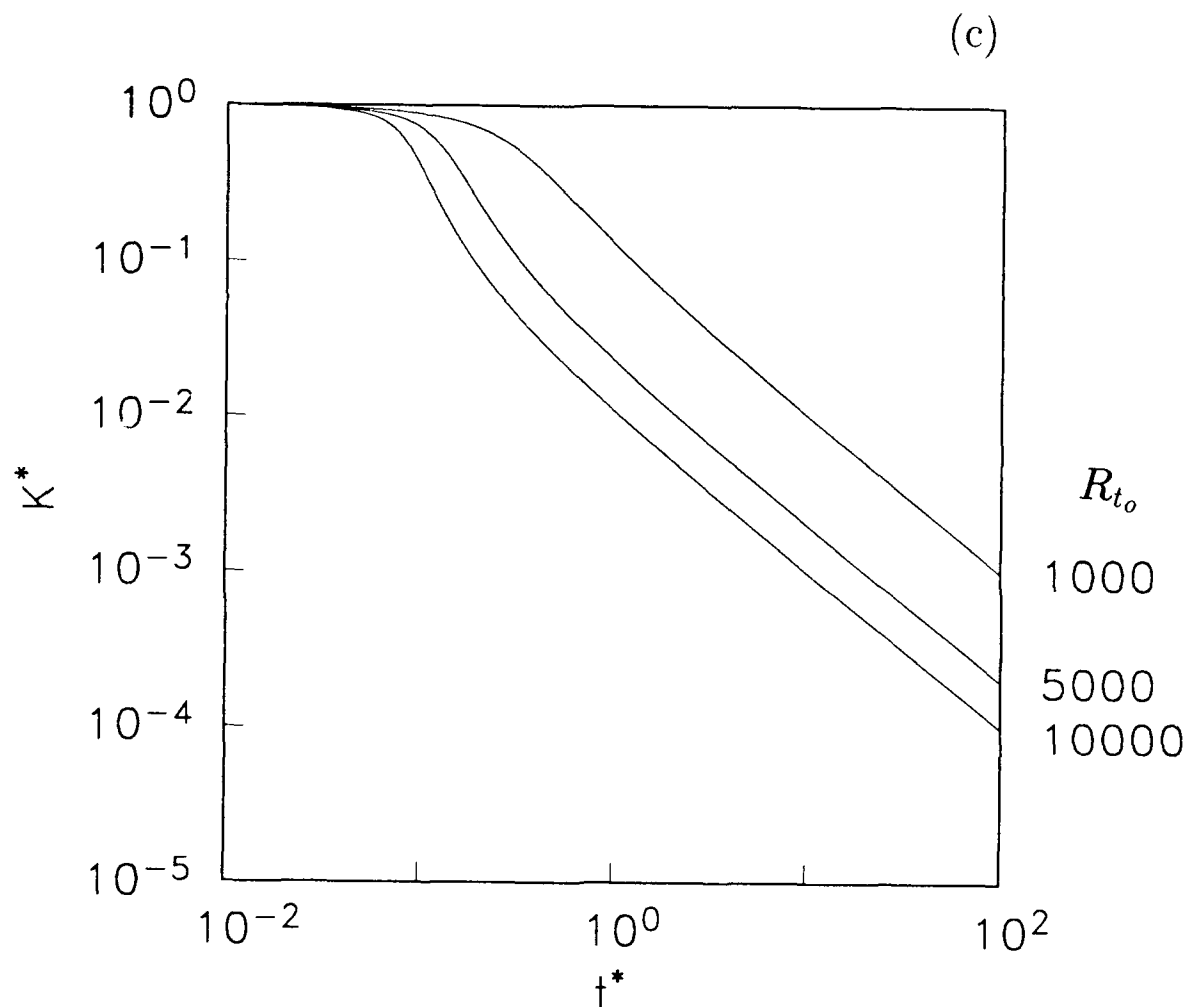
Figure 1. Decay of turbulent kinetic energy in complete self-preserving isotropic turbulence for initial turbulence Reynolds numbers R_{to} = 1000, 5000 and 10,000 : (a) C_{\epsilon_2} = 1.92 , (b) C_{\epsilon_2} = 5 , and (c) C_{\epsilon_2} = 8 .
