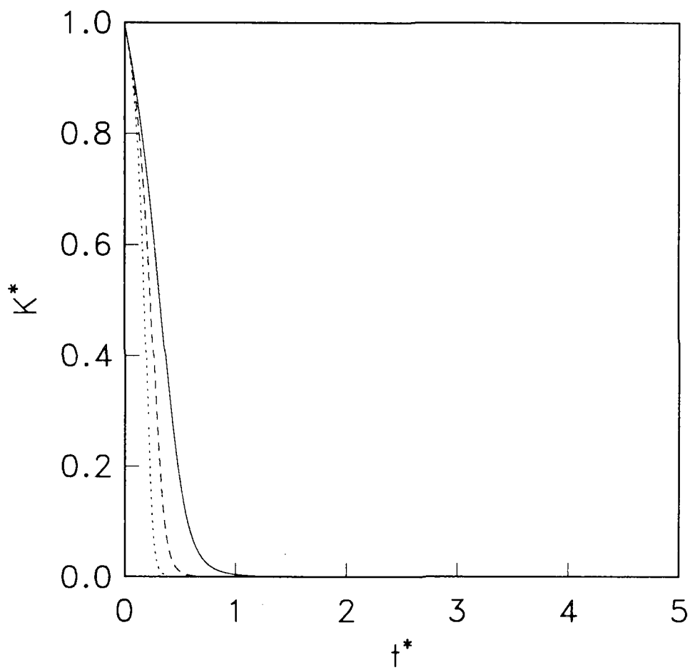
Figure 6. Decay of turbulent kinetic energy in self-preserving isotropic turbulence for C_{e_2} = 1.4 : — R_{t_o} = 200 ; — — R_{t_o} = 500 ; - - - R_{t_o} = 1000 .
