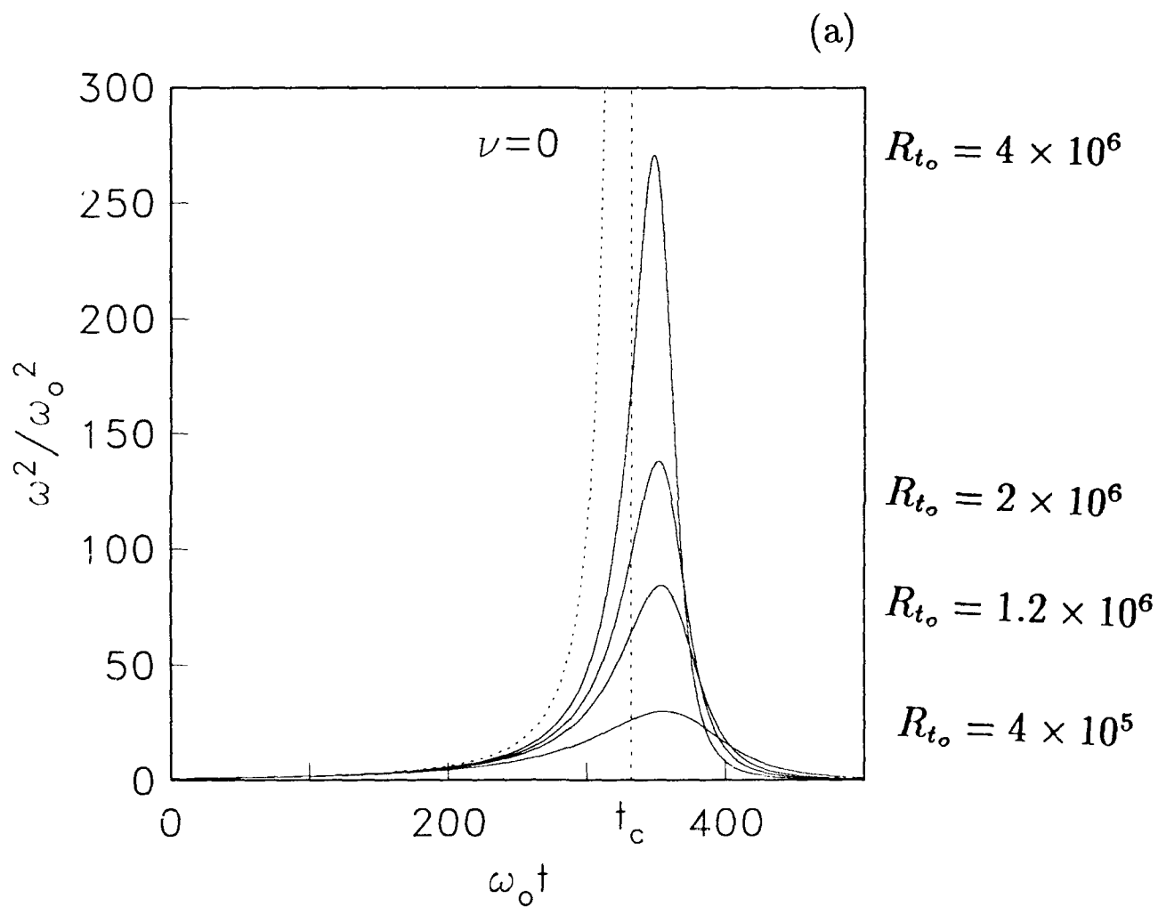
Figure 11. Time evolution of the enstrophy at high turbulence Reynolds numbers: (a) complete self-preserving solution ( C_{\epsilon_2} \doteq 2 ) and (b) schematic from Lesieur (1990) based on EDQNM.
