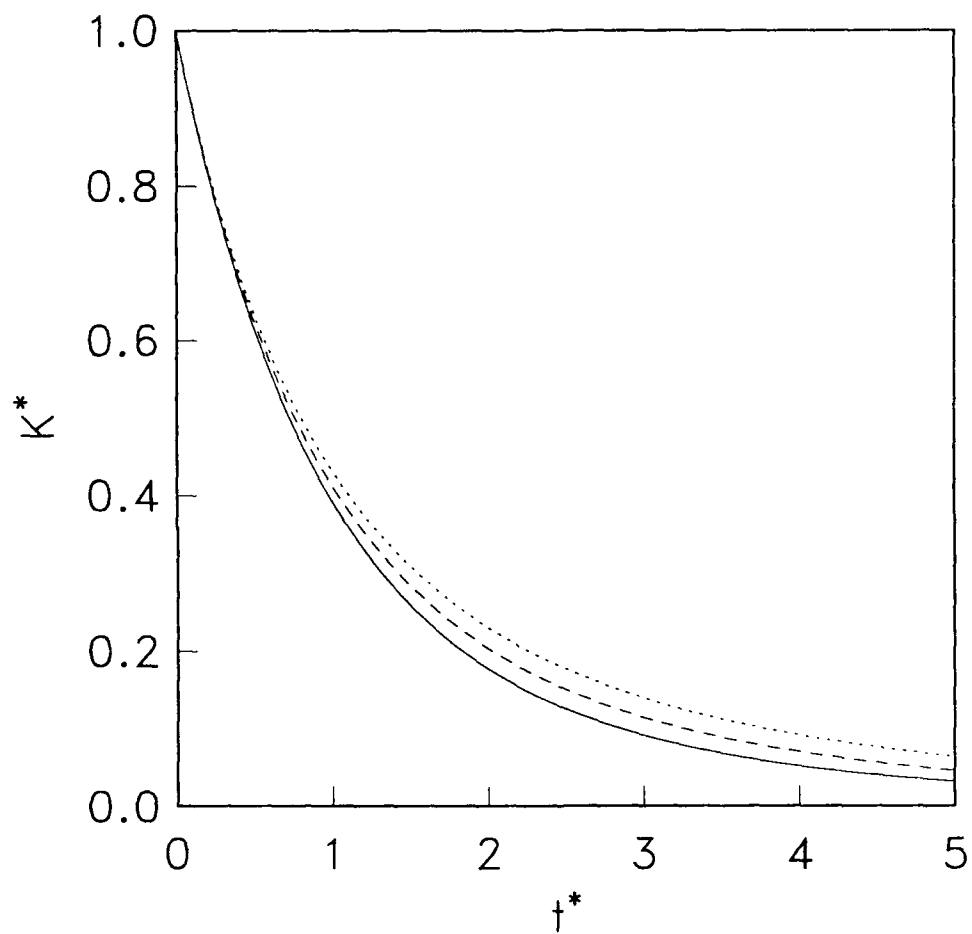
Figure 5. Self-preserving isotropic turbulence at low turbulence Reynolds numbers ( C_{\epsilon_2} = 1.4 ) :— R_{to} = 1 ; — — R_{to} = 0.25 ; - - - Eq. (31).
