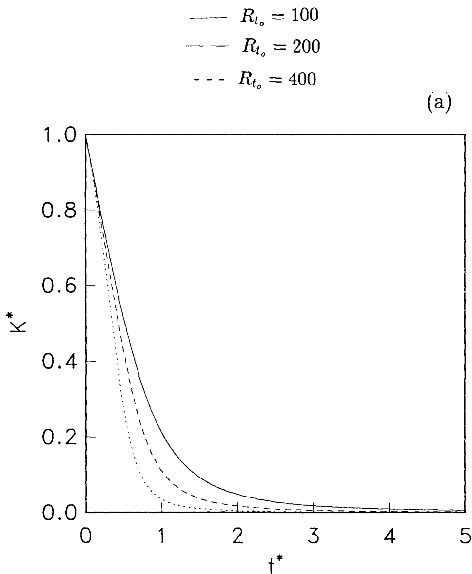
Figure 4. Decay of self-preserving isotropic turbulence for C_{\epsilon_2} = 1.83 and R_{t_o} = 100, 200 and 400: (a) turbulent kinetic energy, and (b) turbulent dissipation rate.
