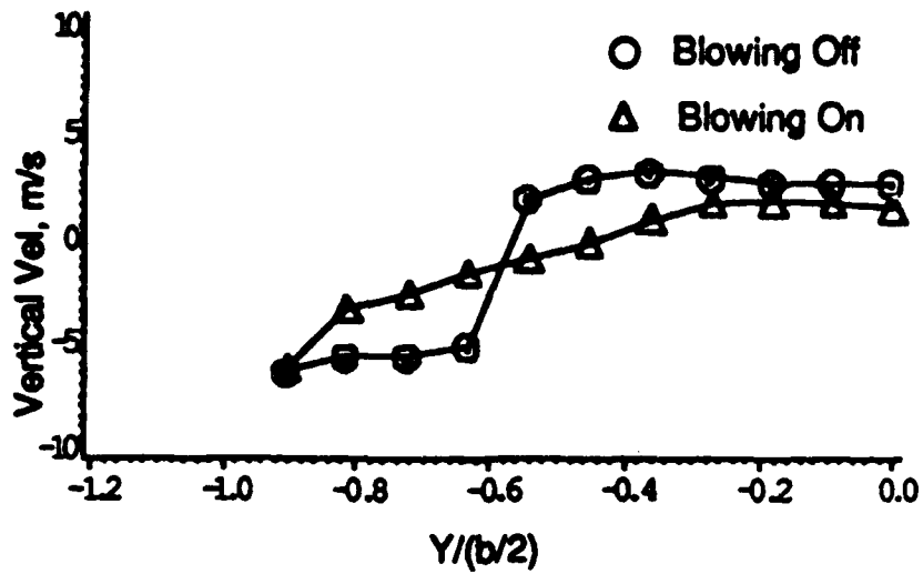
c) mean vertical velocity versus spanwise locations, z/(b/2)=0.57
