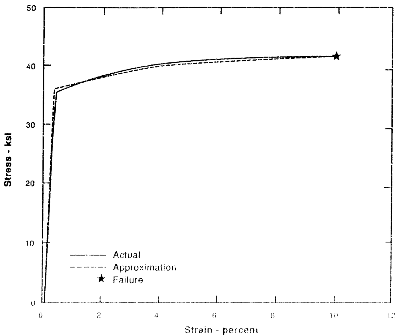
Figure B-20. Typical tensile stress-strain curve for 6061-T6 aluminum alloy and piecewise, linear approximation to curve.
