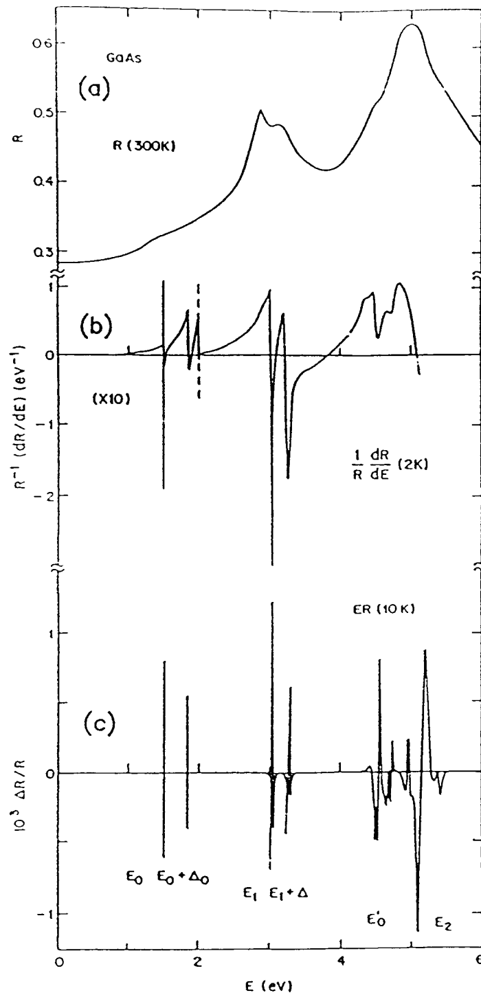
Figure 1. A comparison of three types of GaAs spectra: (a) reflectance R ; (b) energy-derivative reflectance; (c) low-field electroreflectance (Ref. [50]).
