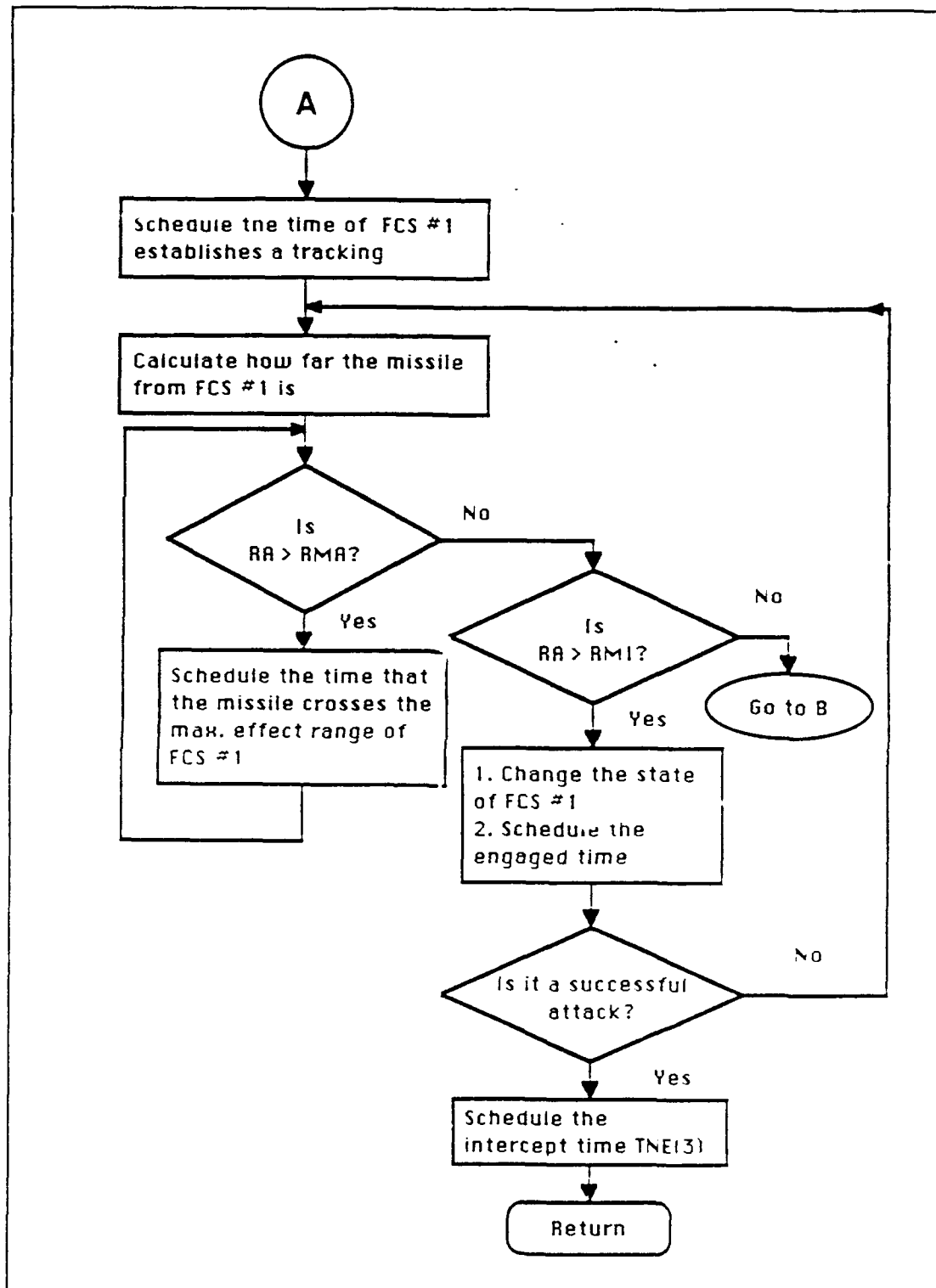
Figure 6 The flowchart of subroutine ENG - A
