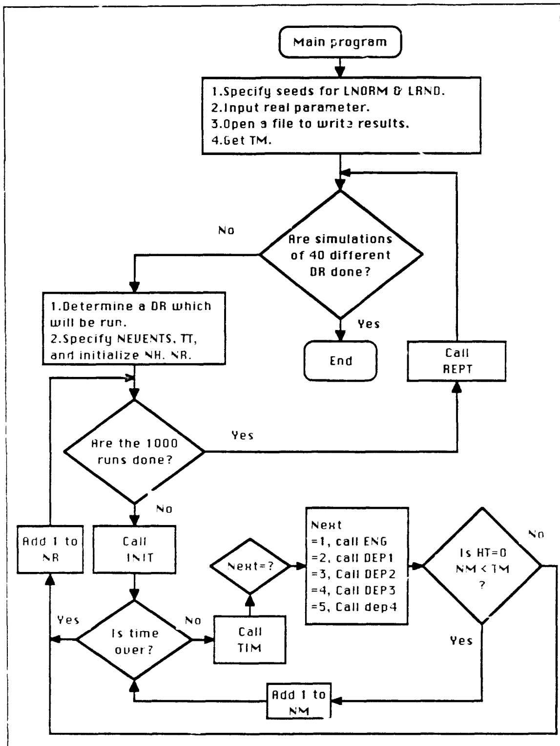
Figure 2 The flowchart of the MAIN PROGRAM
