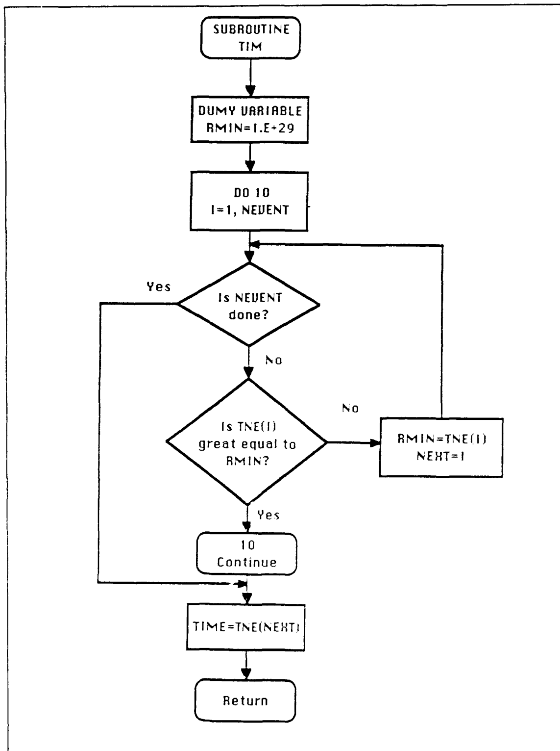
Figure 4 The flowchart of subroutine TIM
