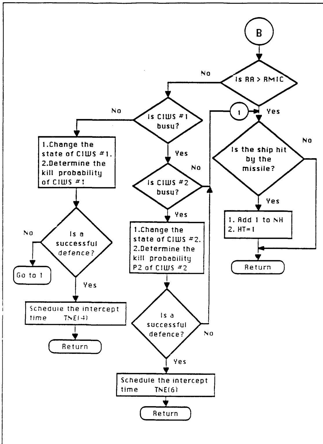
Figure 7 The flowchart of subroutine ENG - B
