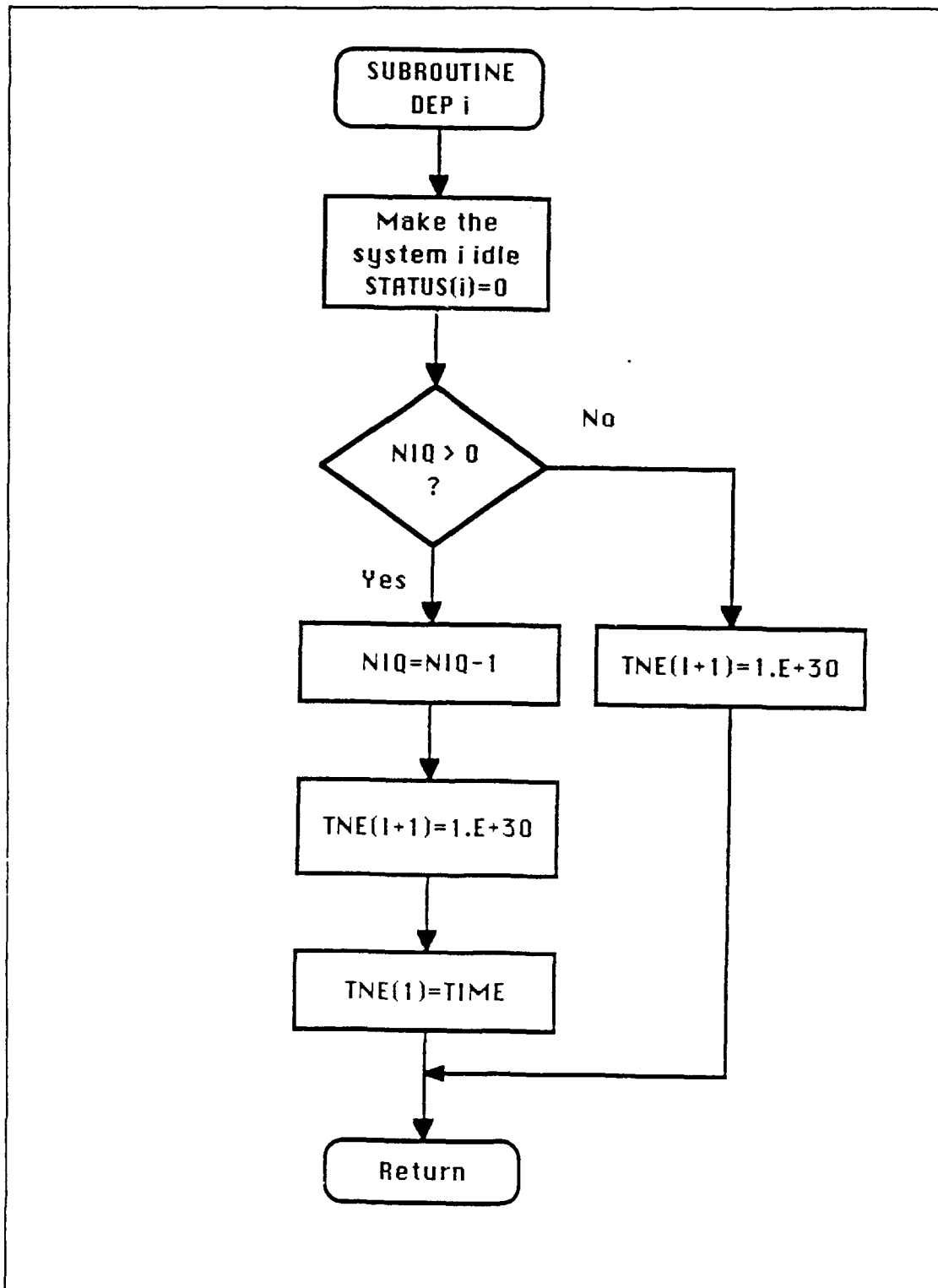
Figure 8 The flowchart of subroutine DEP
