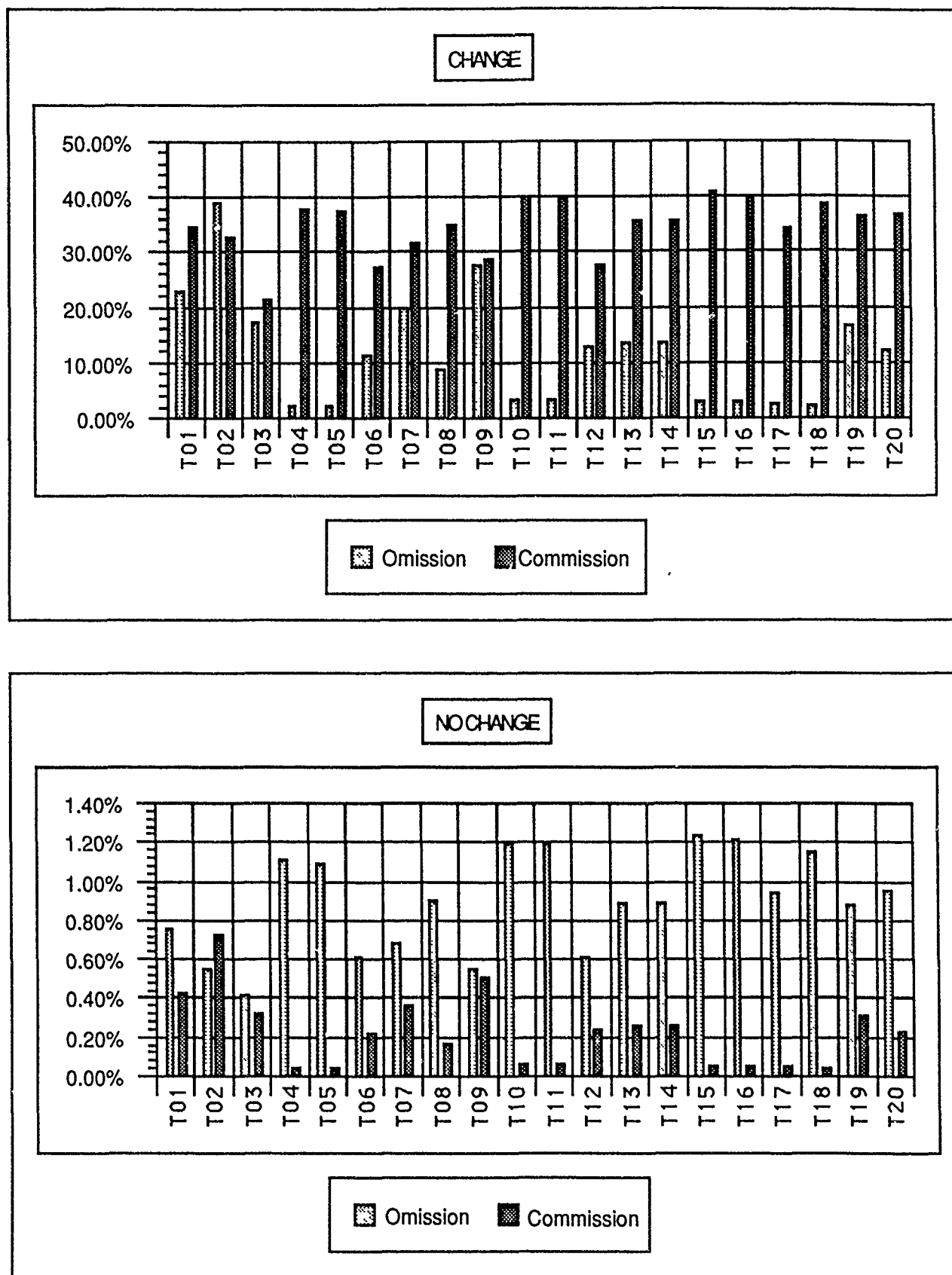
Figure 7. Plots of Omission and Commission Errors During 20 Trials for CHANGE and NO_CHANGE
