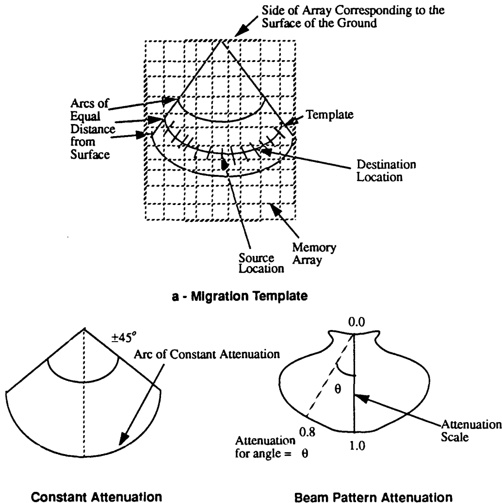
b - Elevation View Review of Antenna Beam Pattern Models
