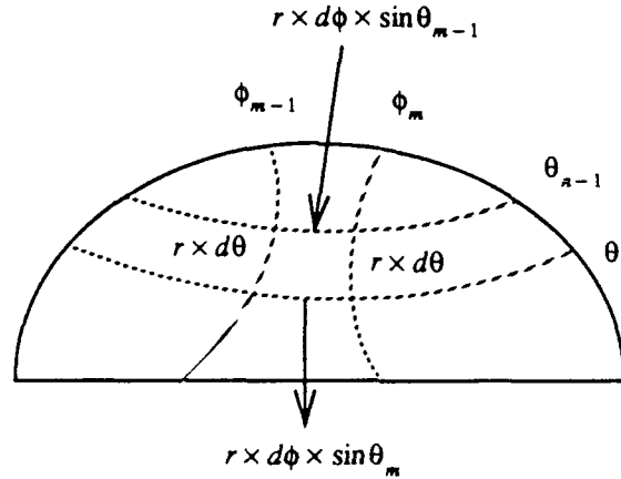
Area of a Trapezoidal Patch
