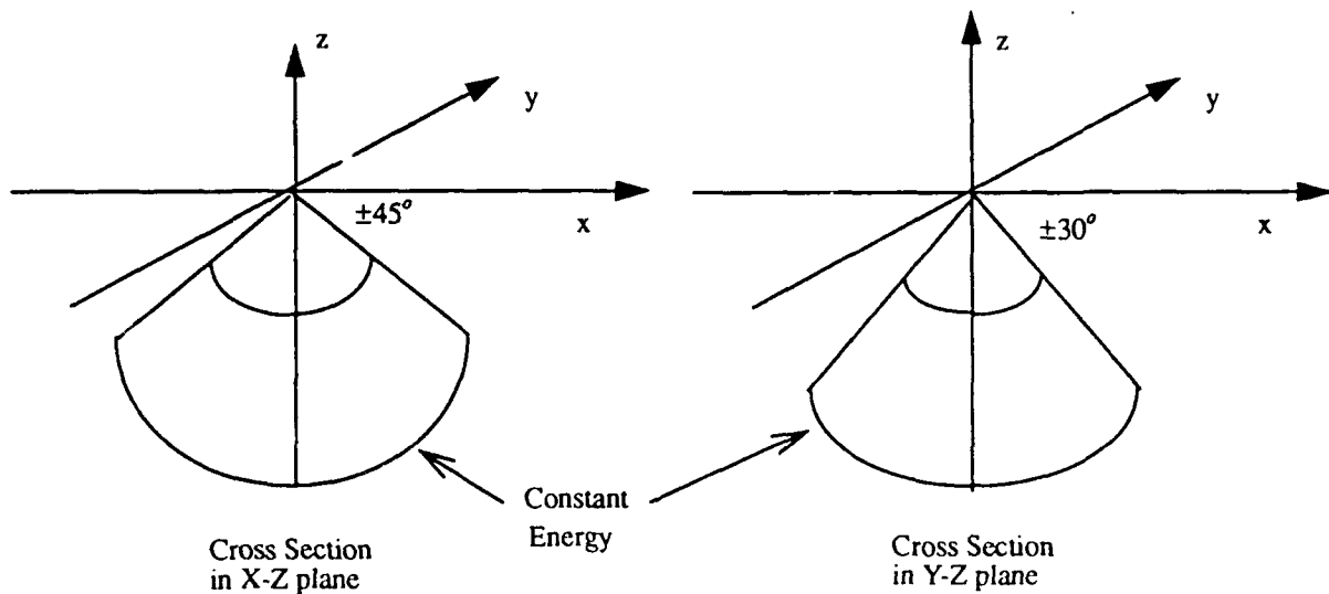
FIGURE 8 Beam Patterns Assuming Constant Energy
