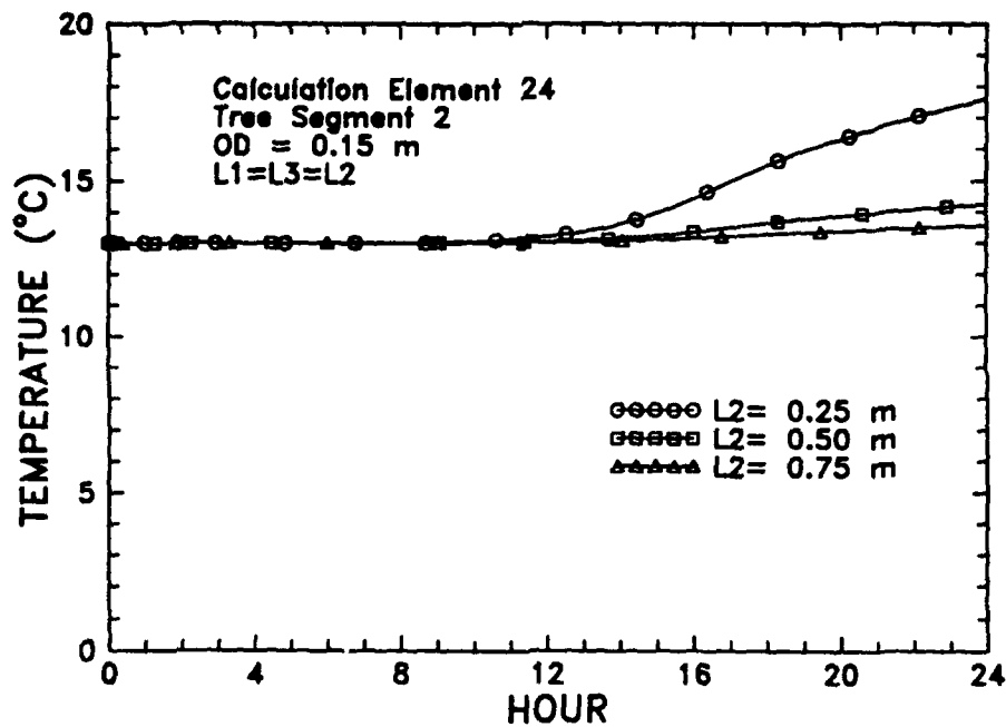
Figure 29. Temperature of Element 24 (OD = 0.15 m) as a Function of Time for Three Different Segment Lengths
