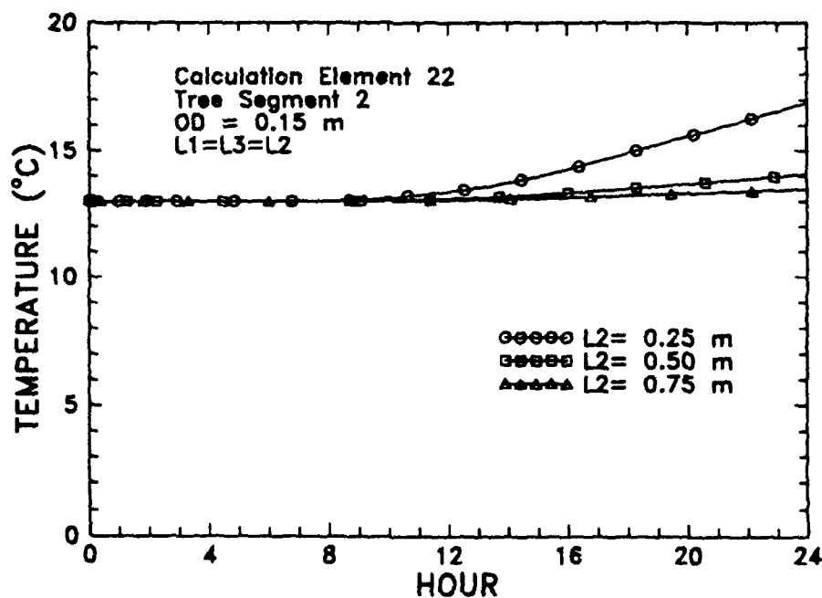
Figure 27. Temperature of Element 22 (OD = 0.15 m) as a Function of Time for Three Different Segment Lengths
