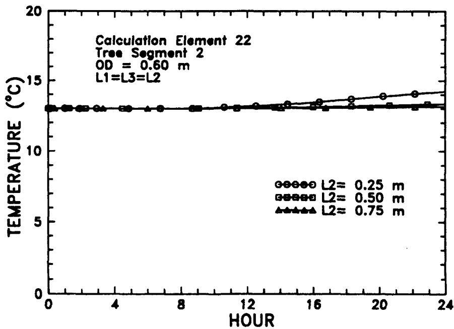
Figure 31. Temperature of Element 22 (OD = 0.6 m) as a Function of Time for Three Different Segment Lengths
