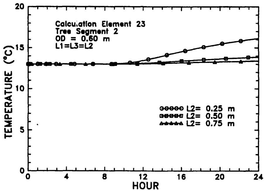
Figure 32. Temperature of Element 23 (OD = 0.6 m) as a Function of Time for Three Different Segment Lengths
