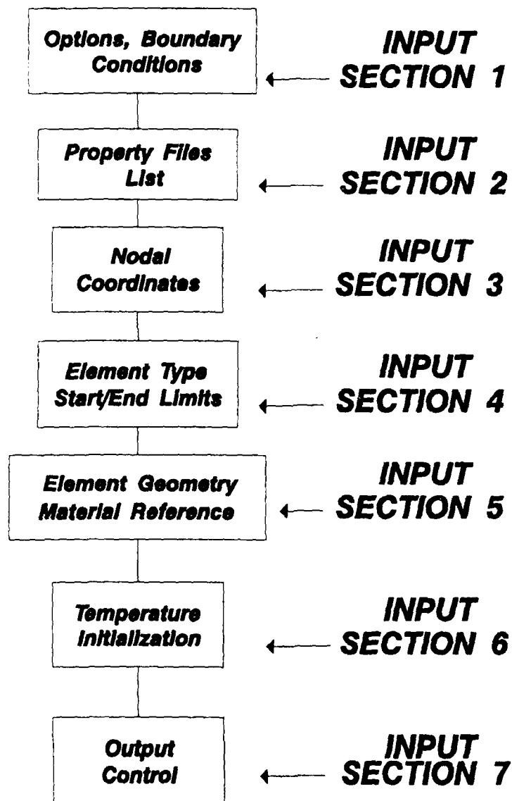
Figure 7. Input Requirements for Multiple Tree Segment Option
