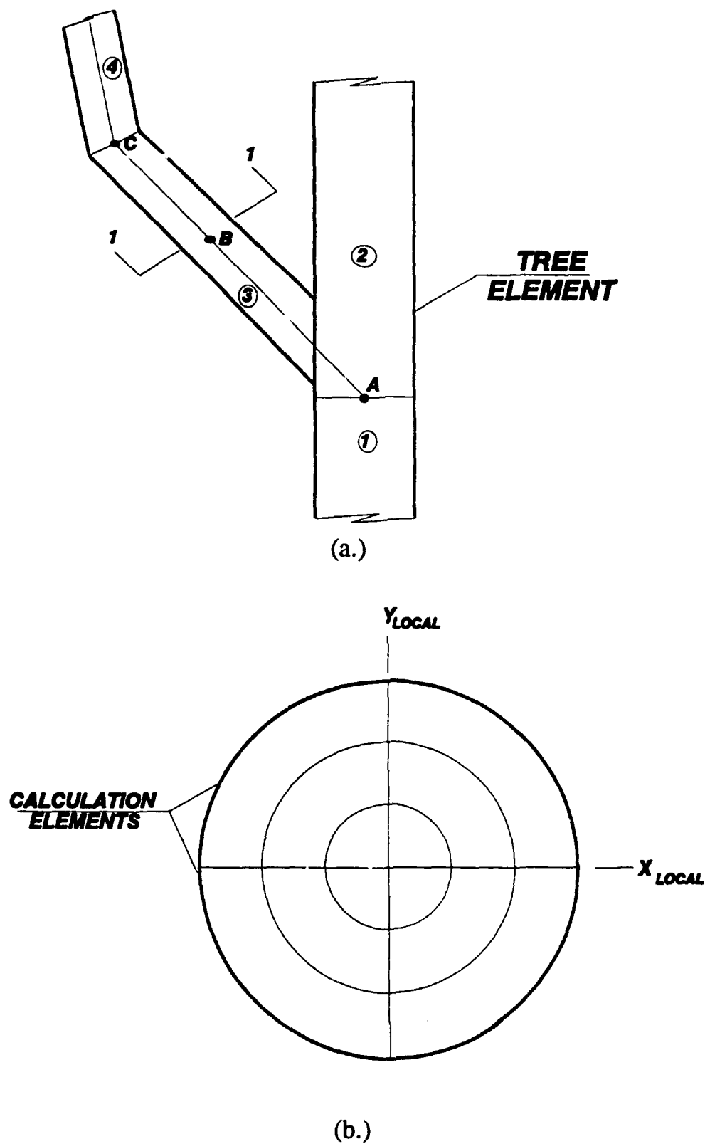
Figure 24. (a.) Typical Branch Connection and (b.) Cross Sectional View of Section 1-1
