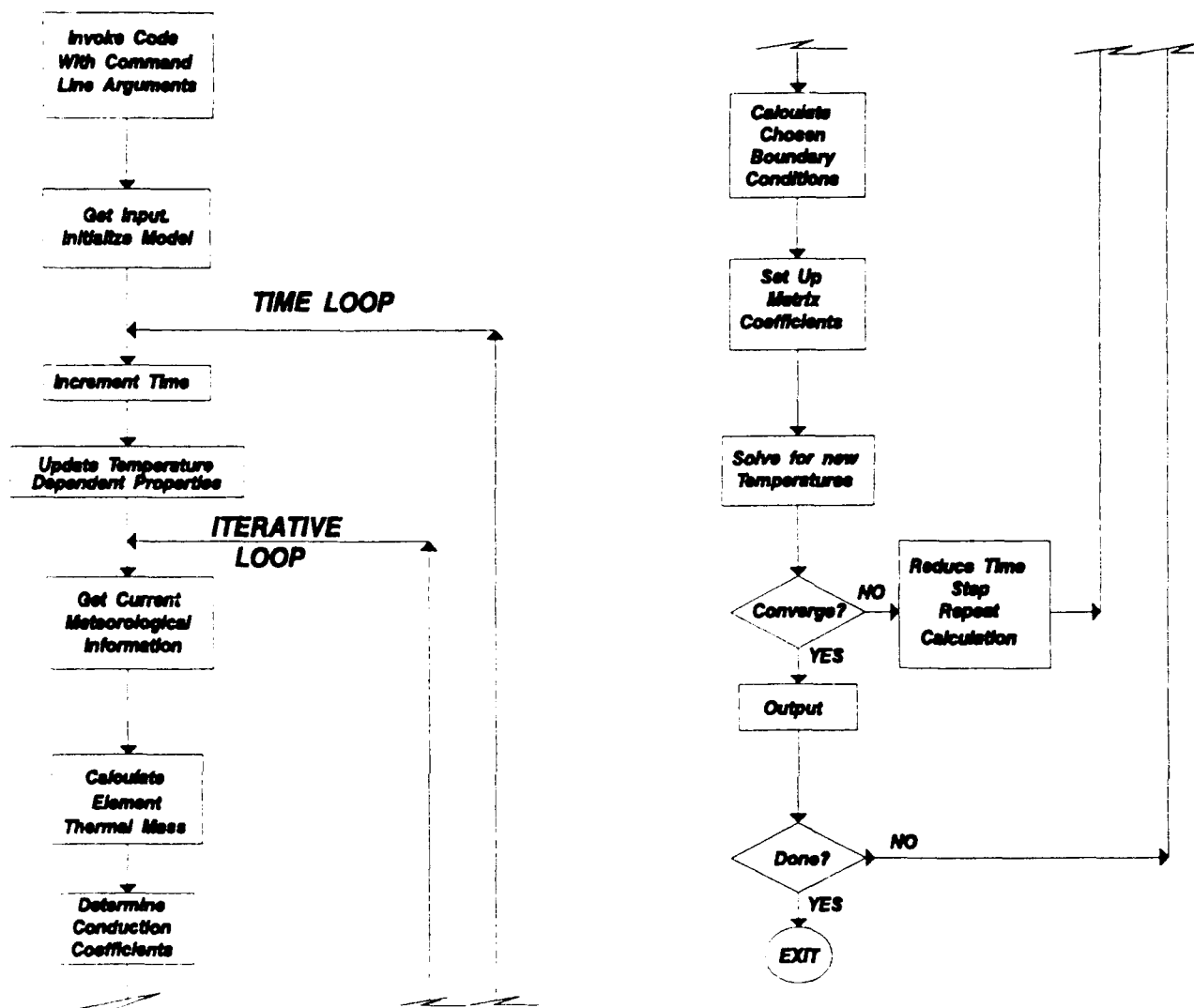
Figure 1. Flowchart of Tree Model Code Execution
