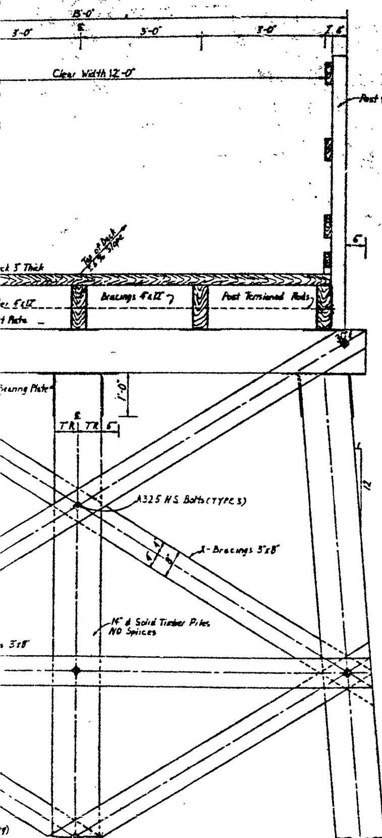
TYPICAL BRIDGE SECTION
