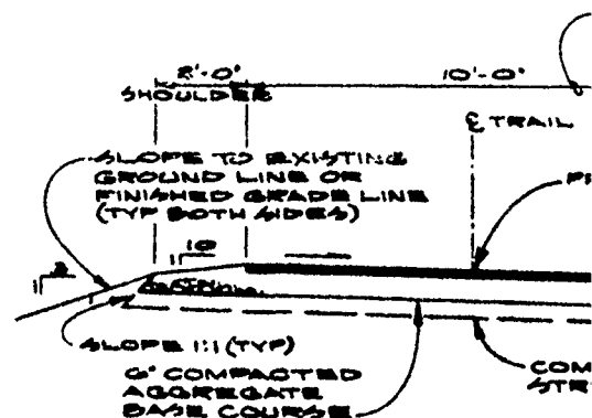
TRAIL SURFACING DETAIL
