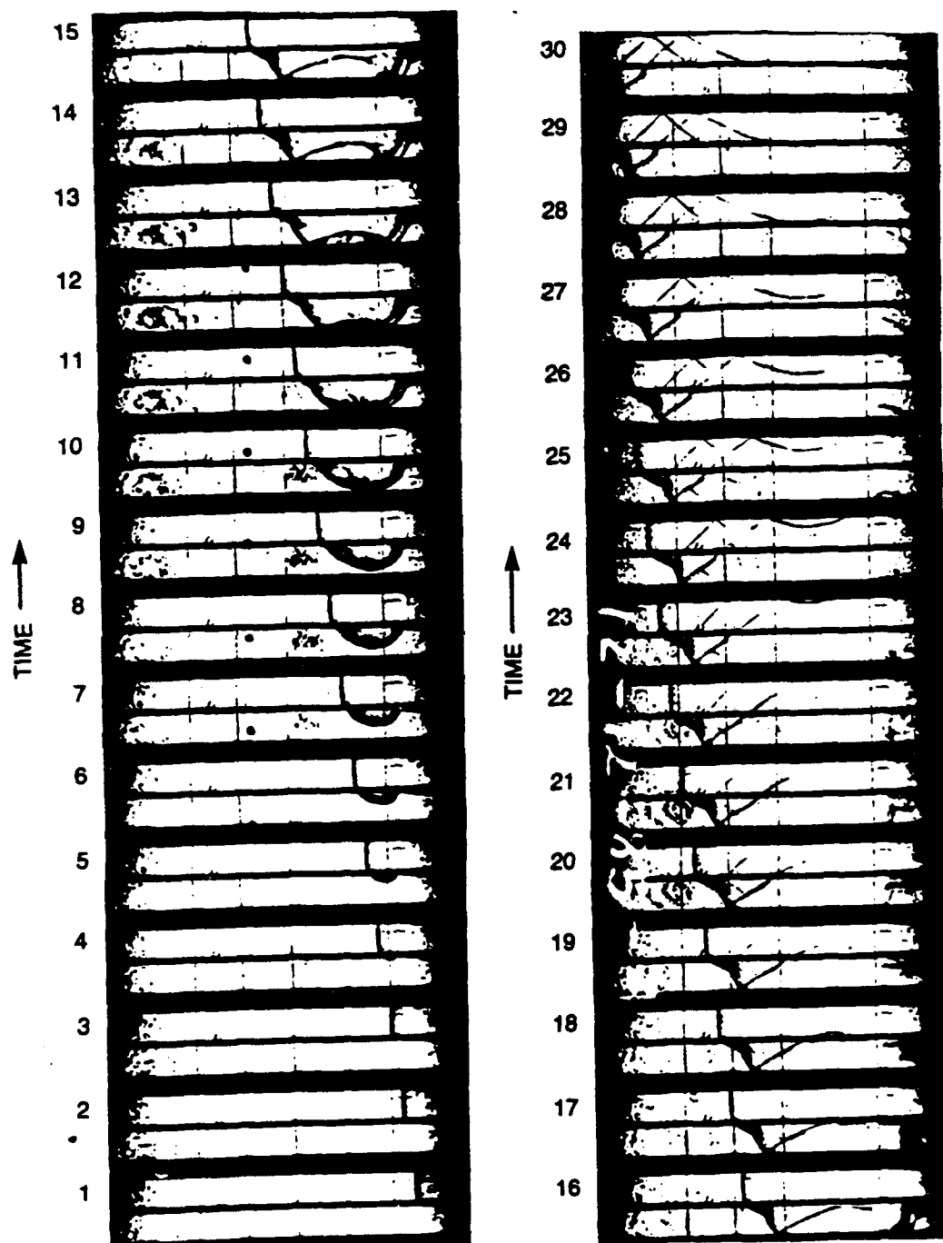
Figure 11. Schlieren photographs for detonation initiated in a stoichiometric primary mixture and a lean bounding mixture. Primary mixture \text{H}_2\text{:O}_2/2:1 ; secondary mixture \text{H}_2\text{:O}_2/0.9:1 , \phi = 0.45 .
