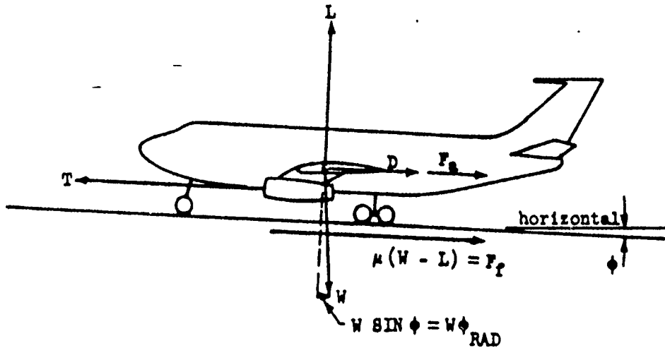
Figure VI.2 Take-off forces
