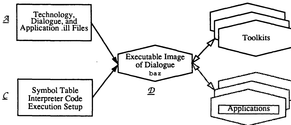
Figure 3-4 – Dialogue Manager
