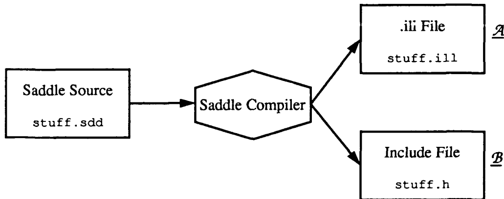
Figure 3-2 – Saddle Compiler
