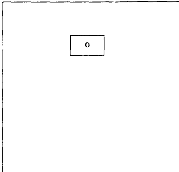
Figure 3-1 Label Widget
