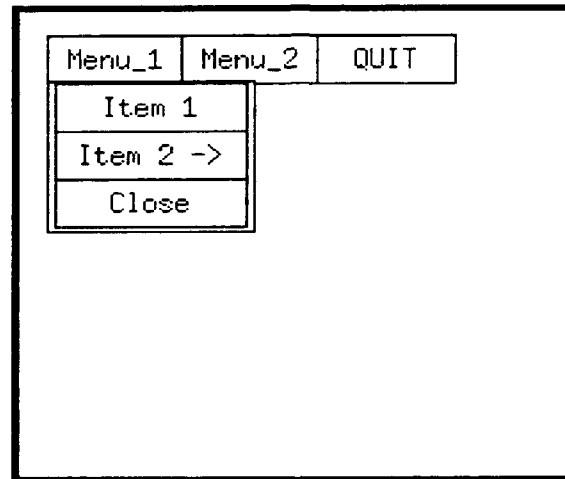
Figure 3-3 Drop-Down Menu
