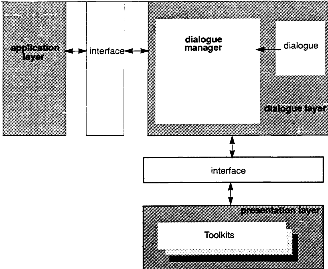
Figure 2-1 Serpent Architecture
