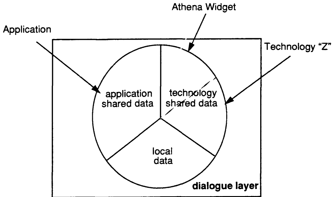
Figure 2-2 Shared Database
