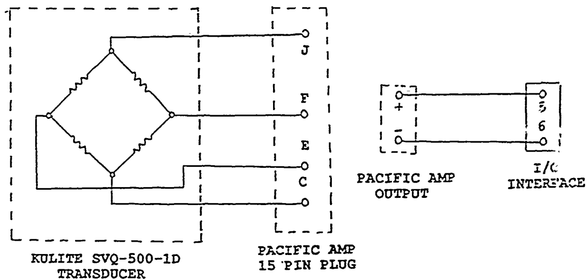
Figure 11. Scanivalve Pressure Acquisition
