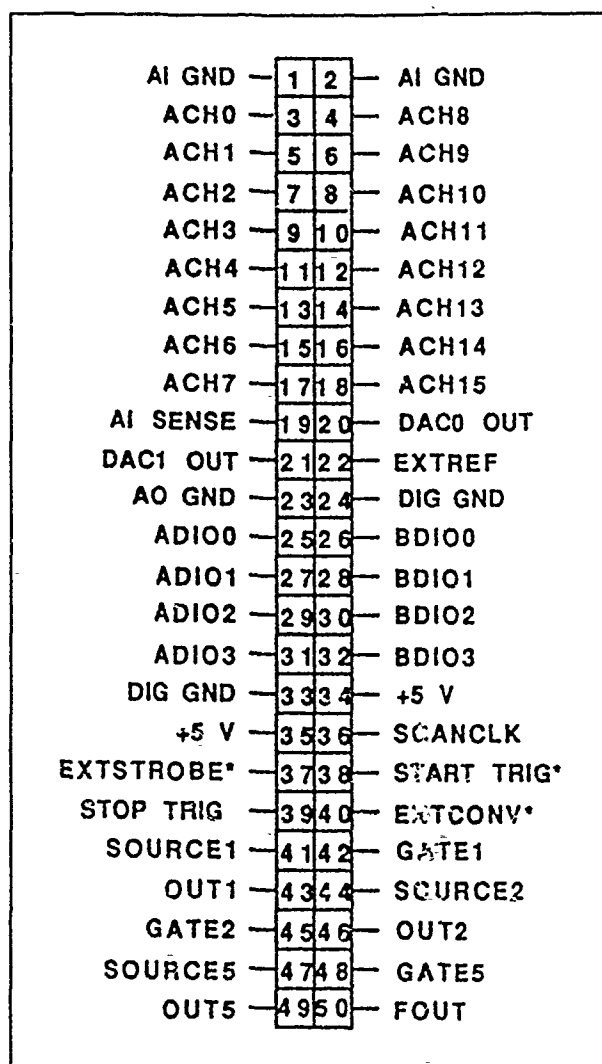
Figure 2. I/O Interface
