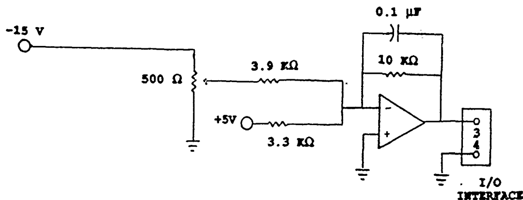
Figure 7. AOA Acquisition
