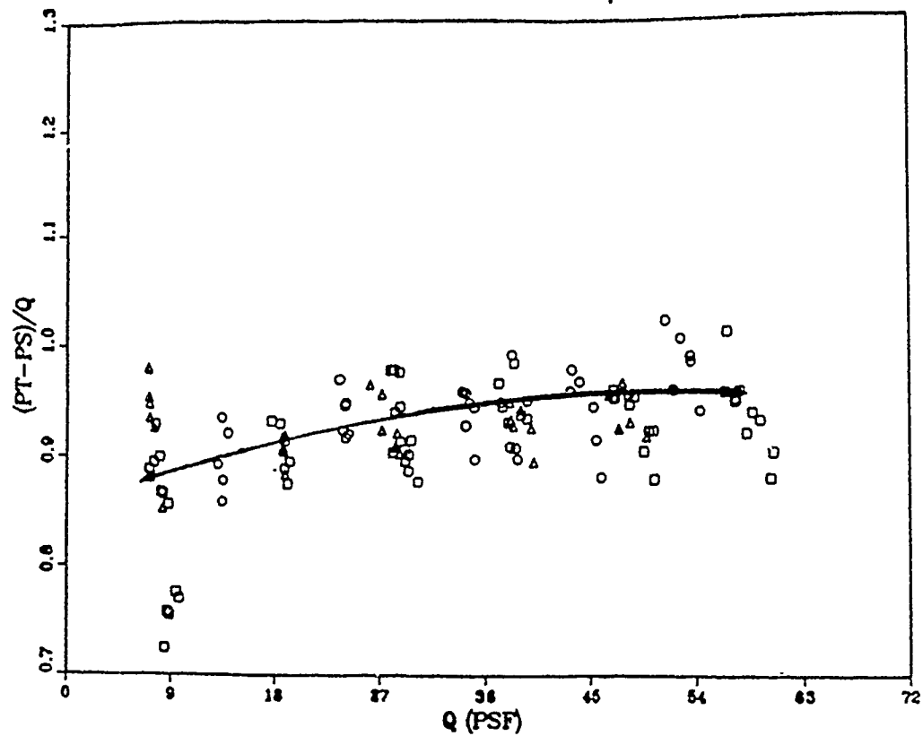
Figure 13. Airspeed Calibration
