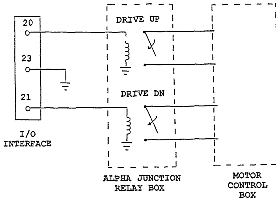
Figure 8. AOA Control
