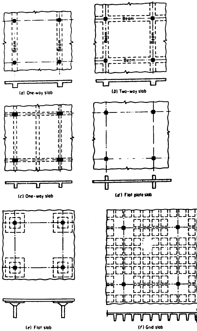
Figure 40. Typical slabs.
