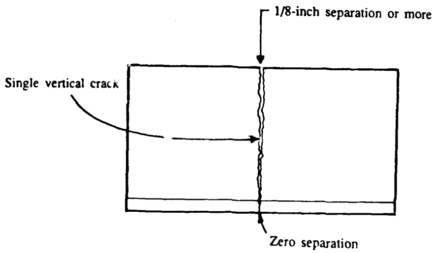
Figure 37. Upward movement of a foundation wall.
