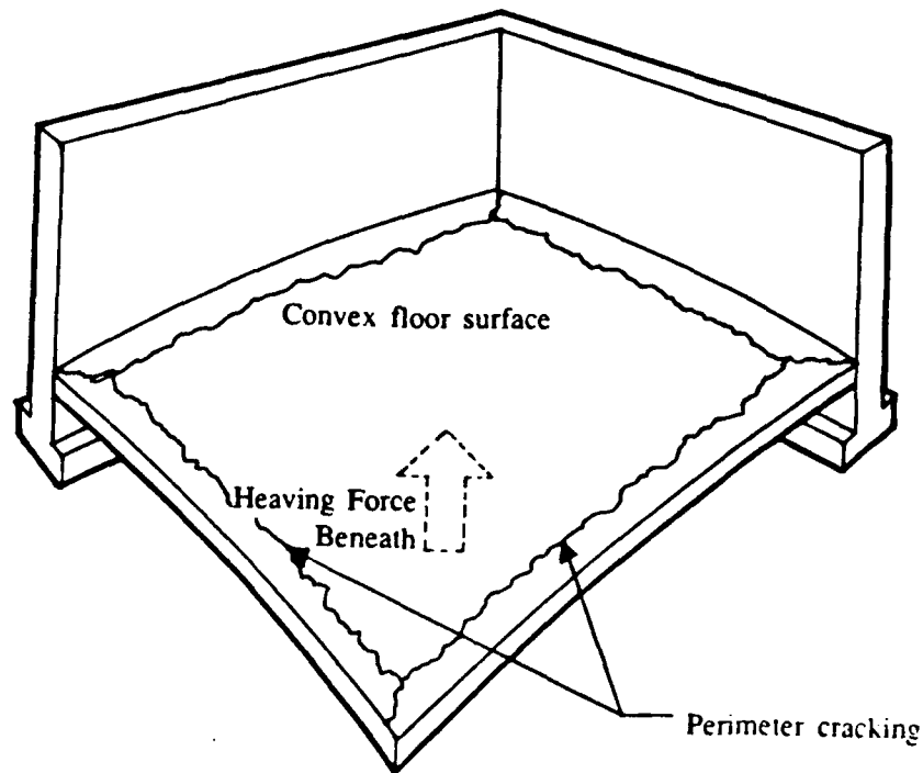
Figure 31. Heaving soil under a floor slab causing a convex floor and perimeter cracking.
