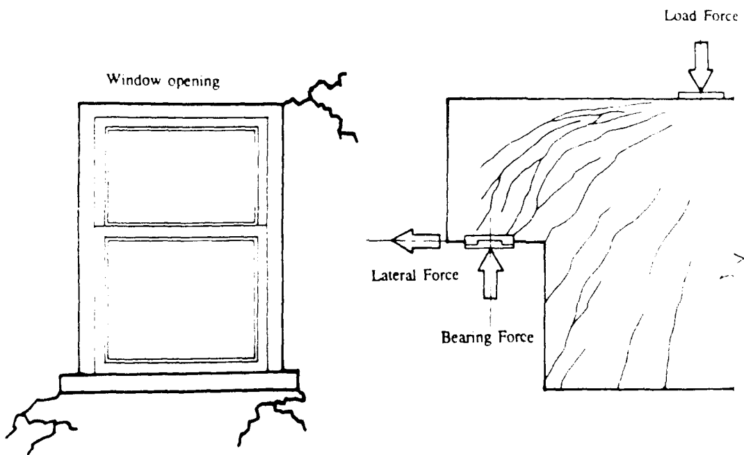
(a) Cracks at reentrant corners.
