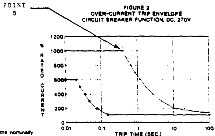
Fig. 2 Over - Current Trip Curves
