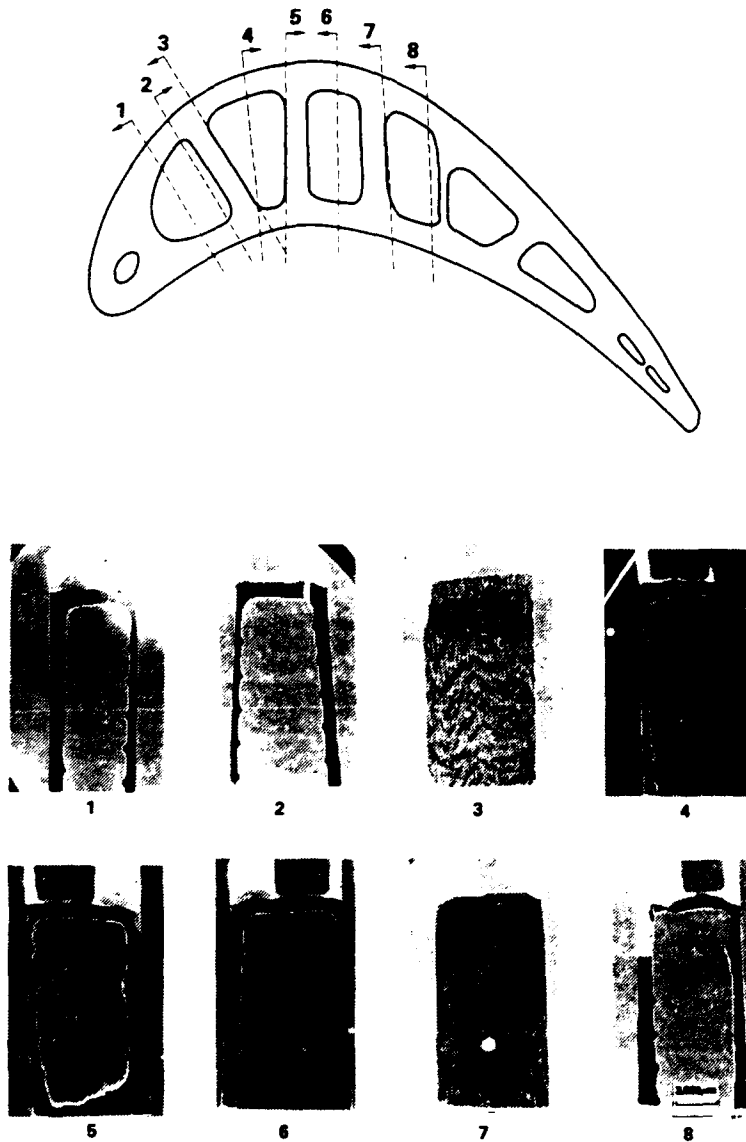
Figure 10. Section views of the microstructure of a DS-R80H blade illustrating the blade-weld interface through the blade cross-section.
