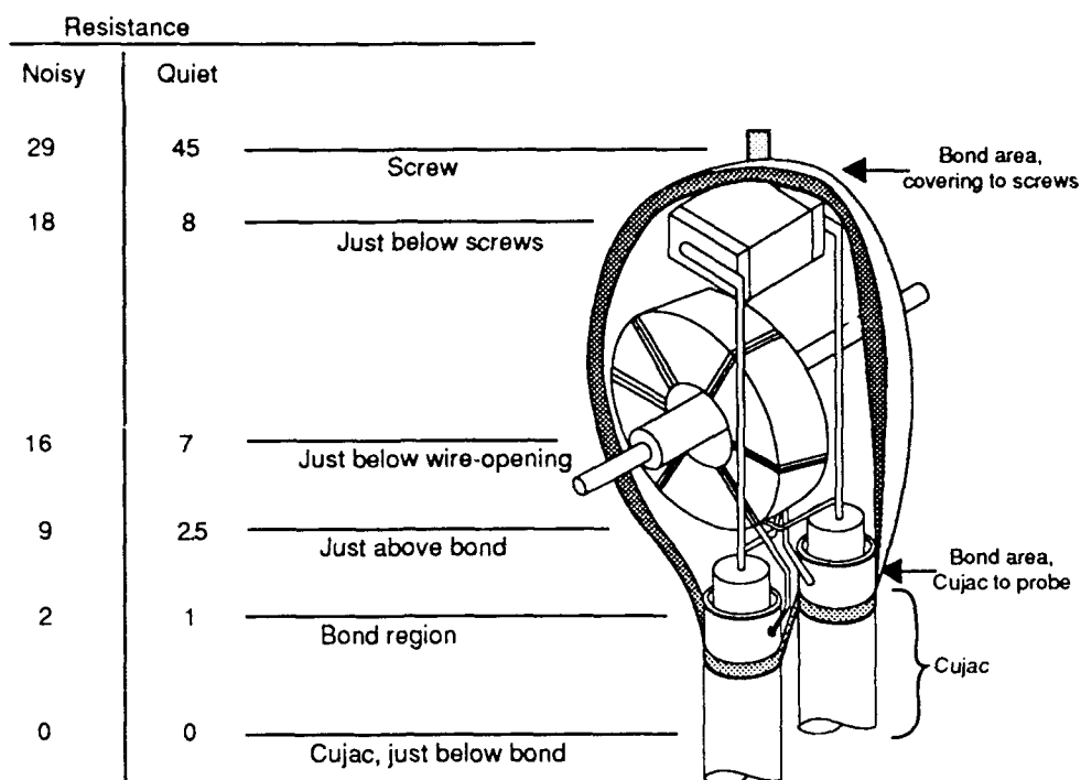
Figure 10. Measurement of resistance of conducting epoxy covering of noisy probe (left) and quiet probe (right).
