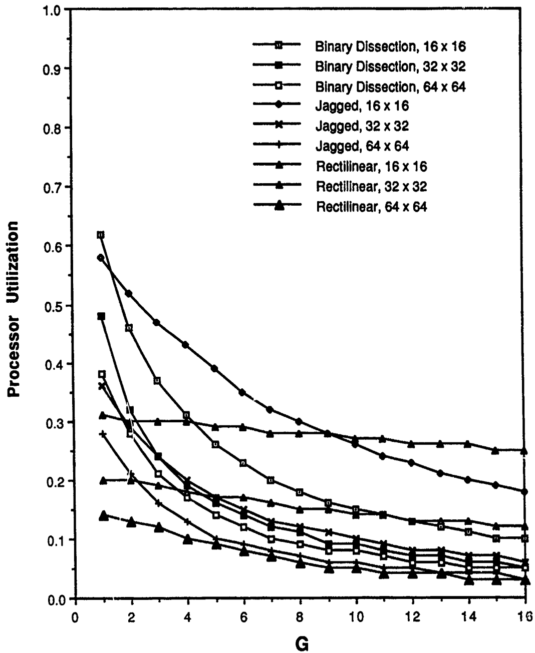
Figure 4: Processor utilizations on the BD, JP, and RP partitions of grid A, for 16 \times 16 , 32 \times 32 , and 64 \times 64 processor arrays
