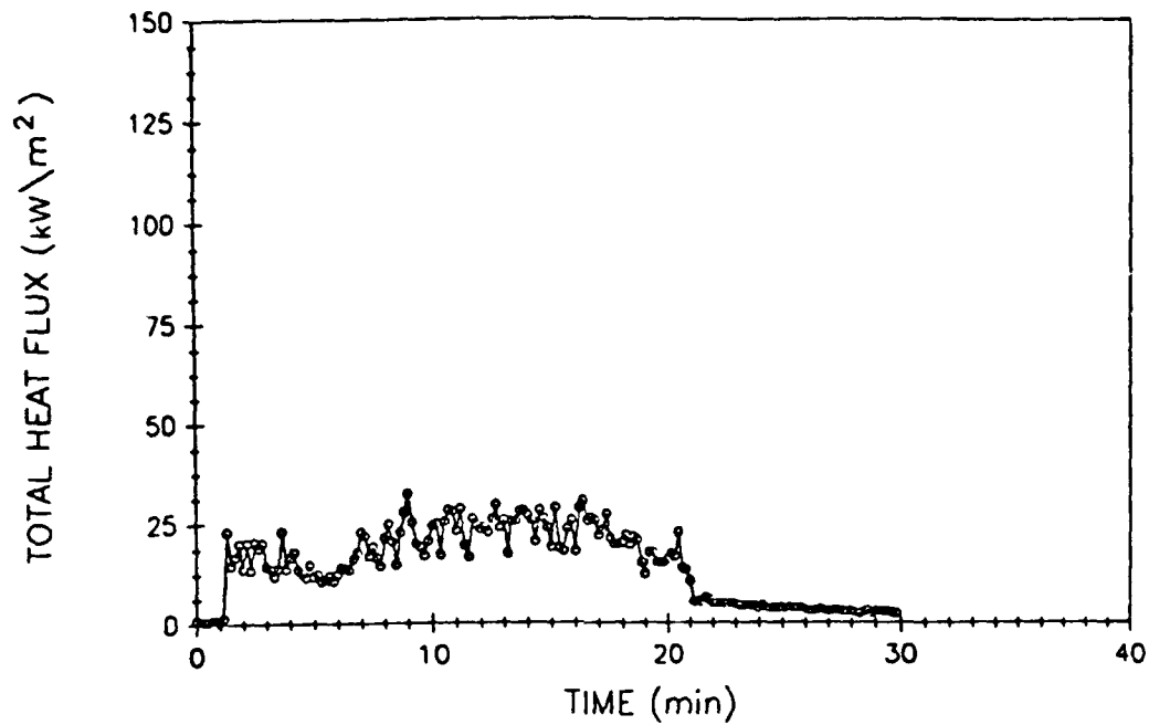
Fig. A32 – Fire compartment total heat flux
