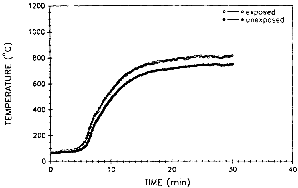
Fig. A71 - East bulkhead average surface temperatures
