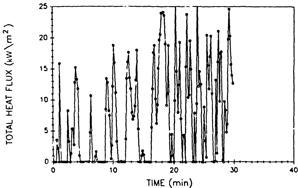
Fig. A23 - West compartment total heat flux
