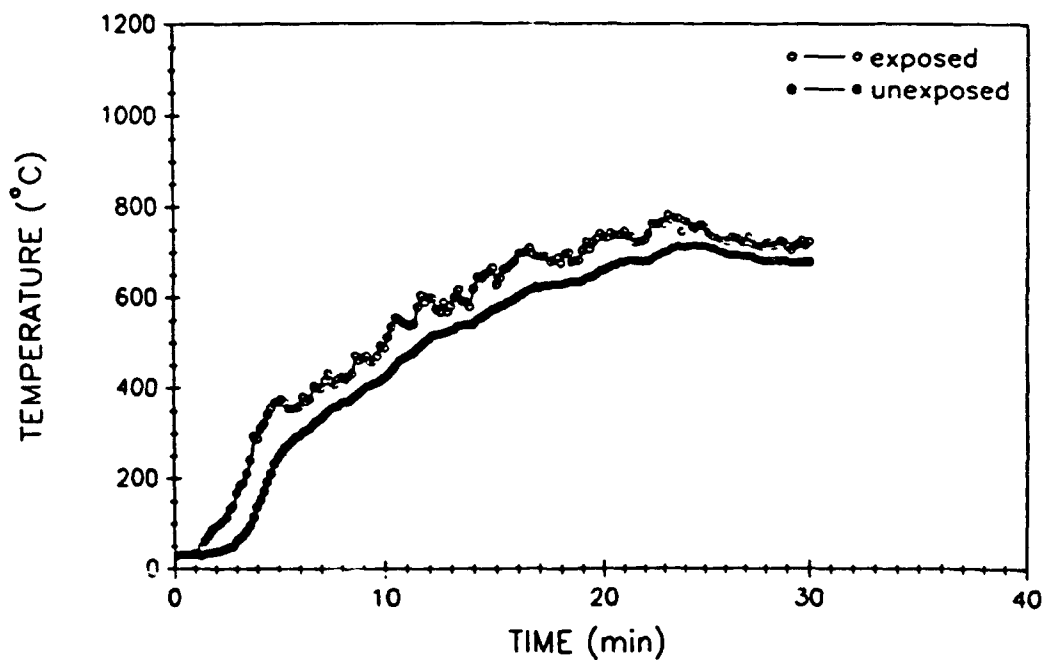
Fig. A57 – West bulkhead average surface temperatures
