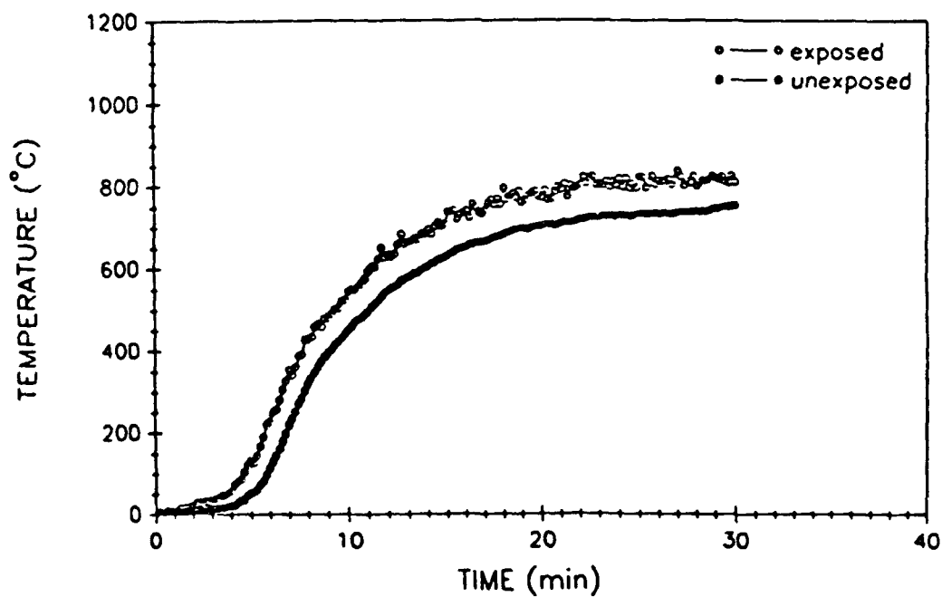
Fig. A87 - West bulkhead average surface temperatures
