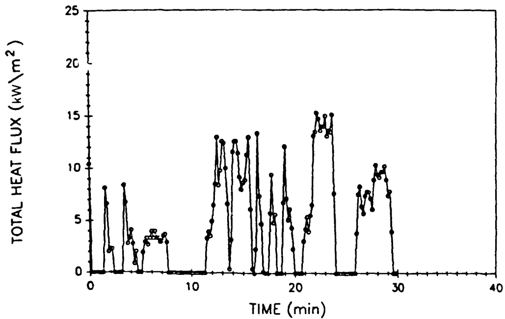
Fig. A6 - East compartment total heat flux
