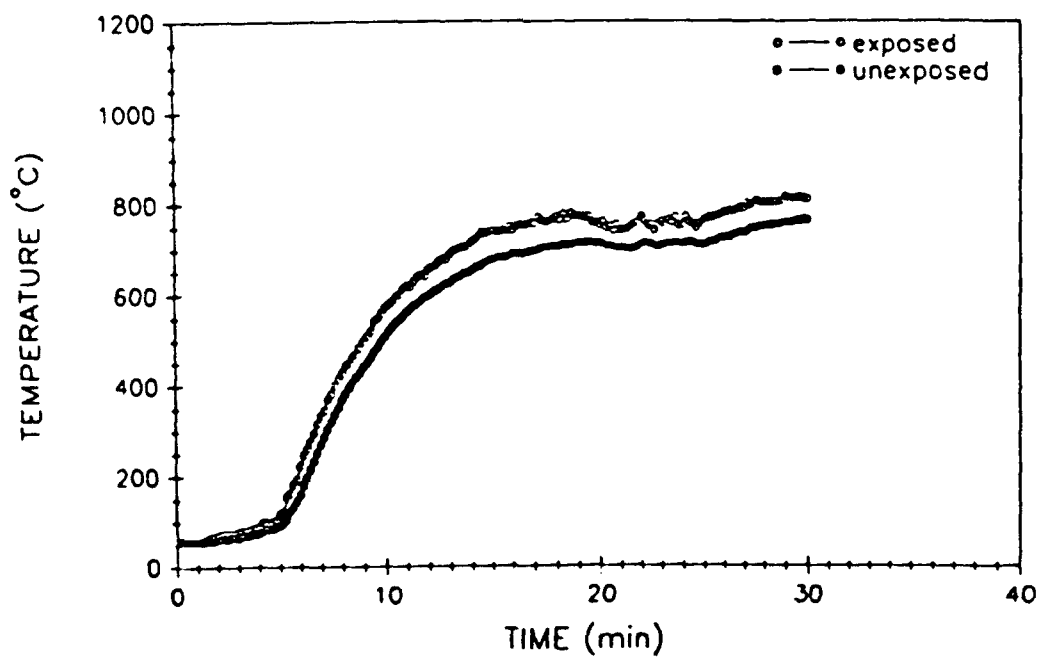
Fig. A101 – East bulkhead average surface temperatures
