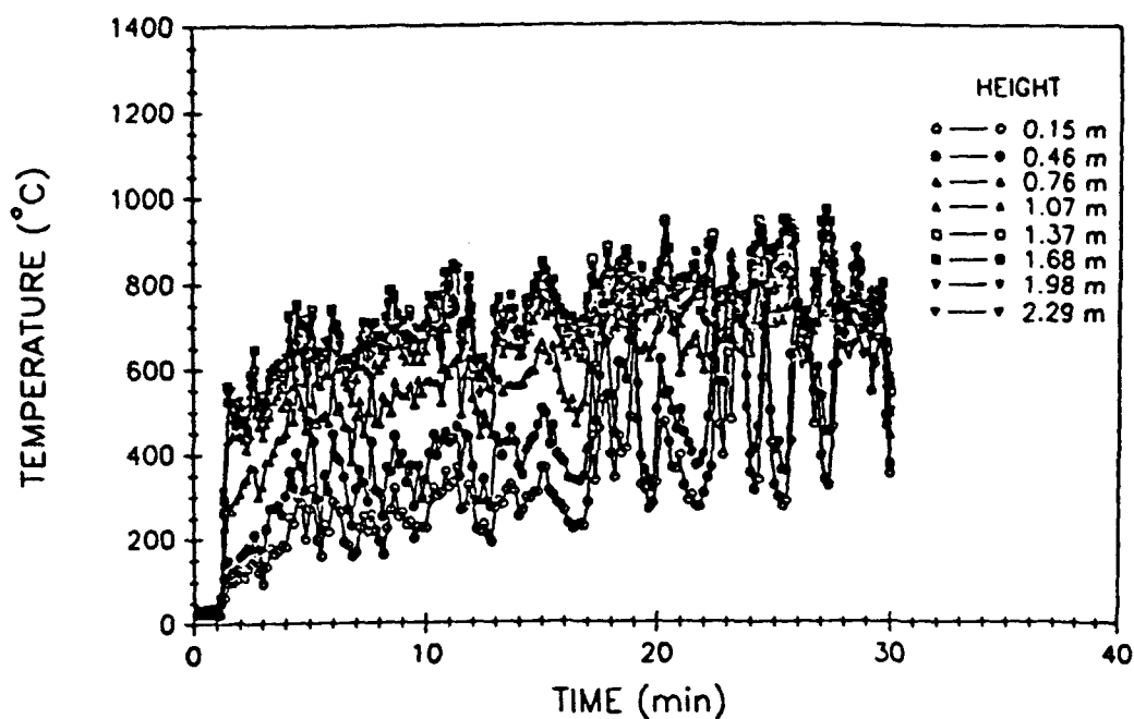
Fig. A16 - Fire compartment air temperatures
