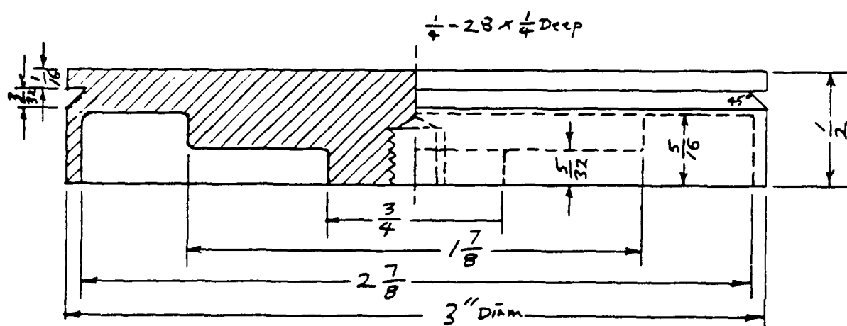
Figure 6 Drawing of the substrate stage utilized to control the temperature profile of the wafers during depositions.
